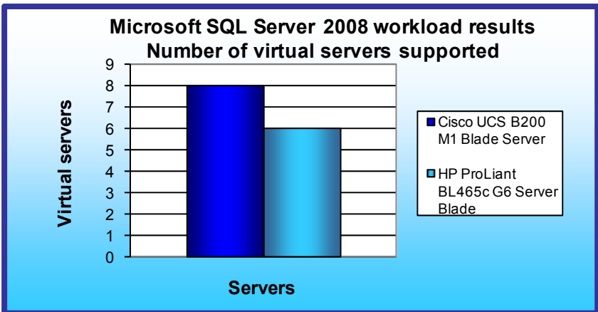
Figure 1: SQL Server consolidation results for the blade servers. Higher numbers are better.
