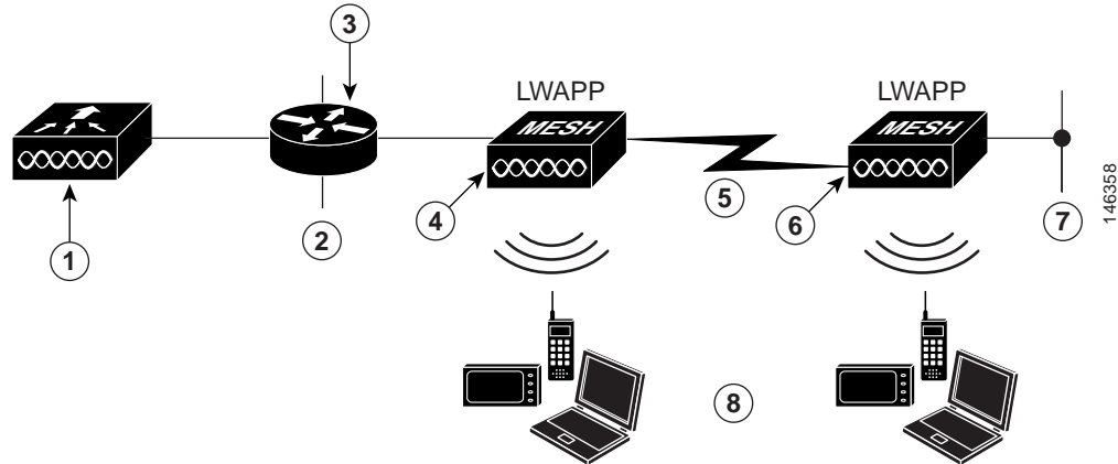
Figure 1-1 Point-to-Point Deployment
