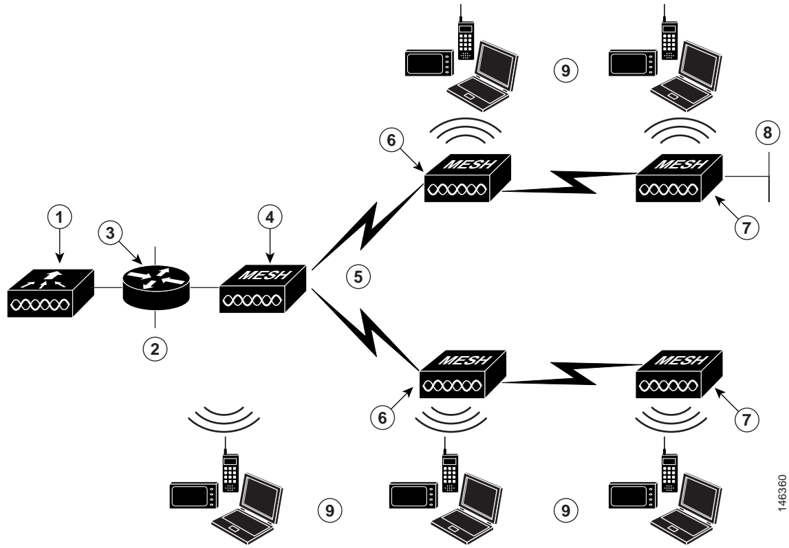
Figure 1-2 Point-to-Multipoint Deployment
