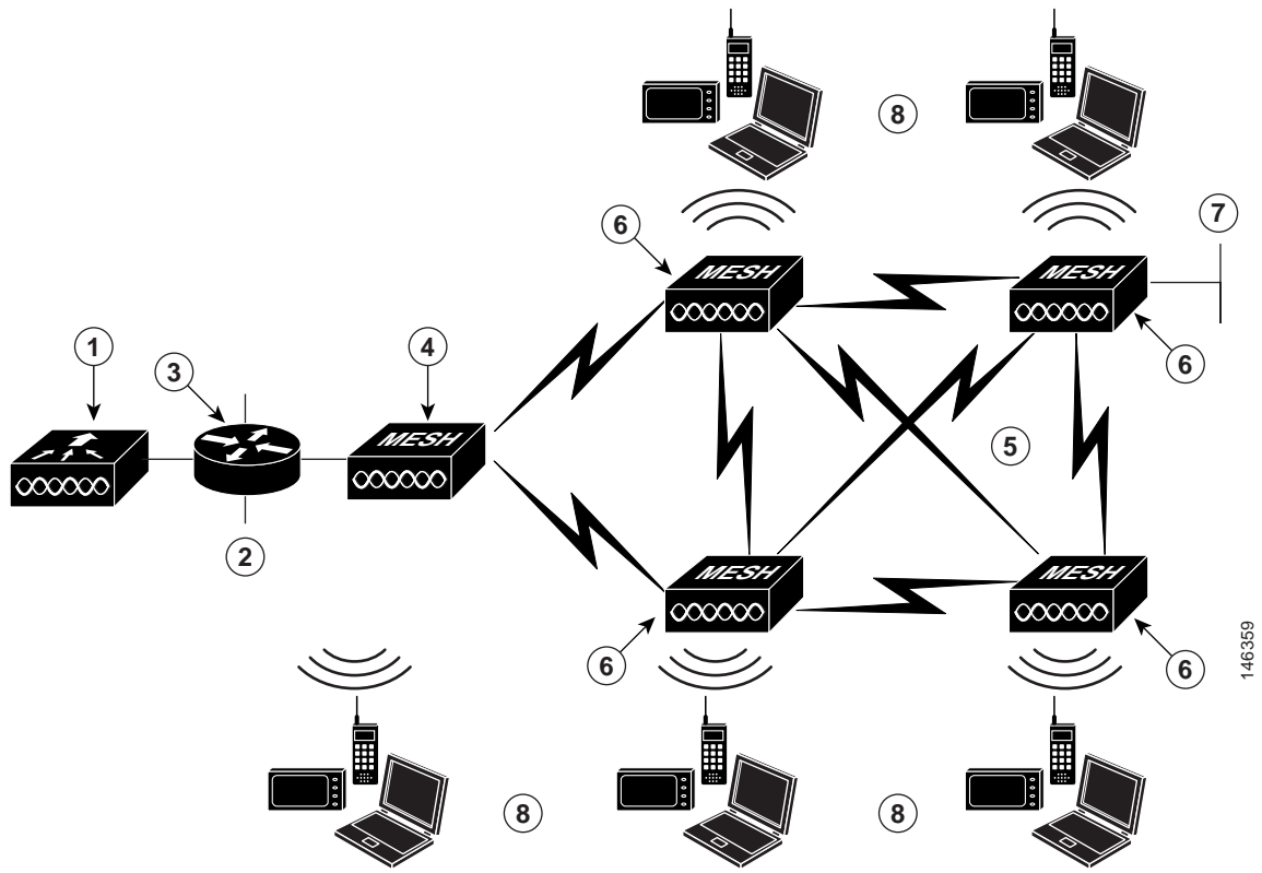
Figure 1-3 Mesh Deployment
