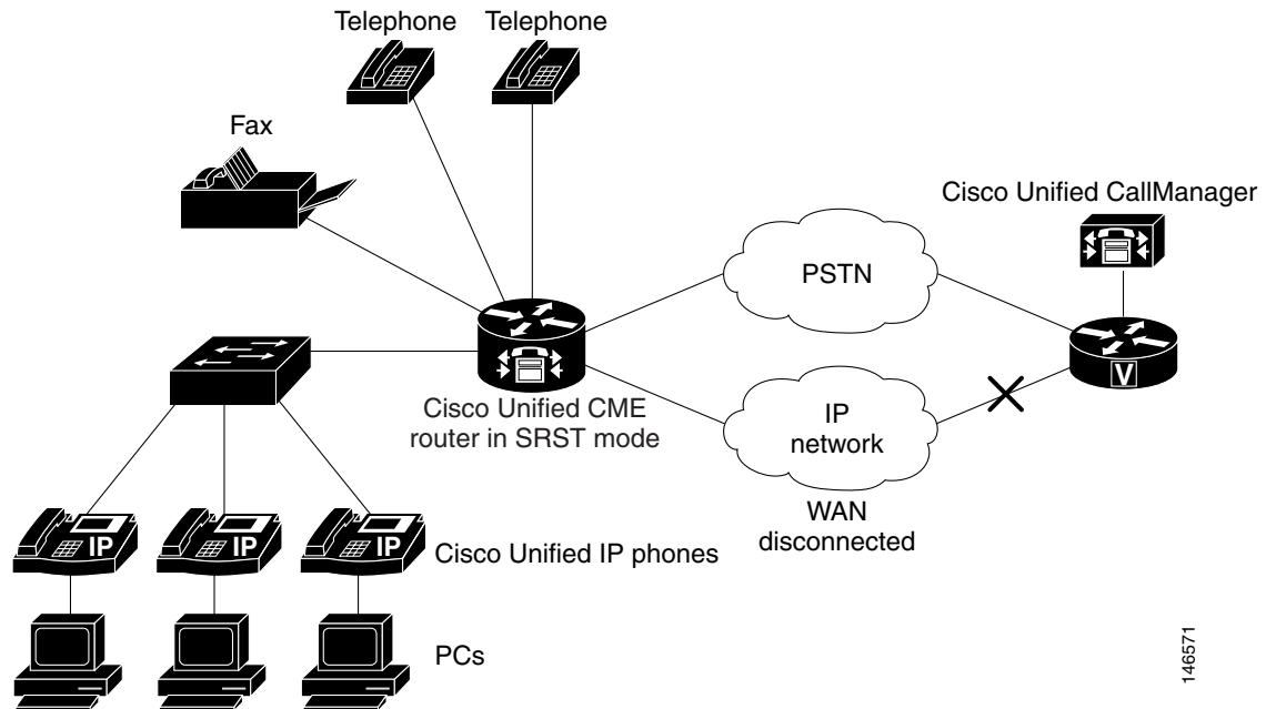
Figure 42 SRST Fallback Support using Cisco Unified CME
