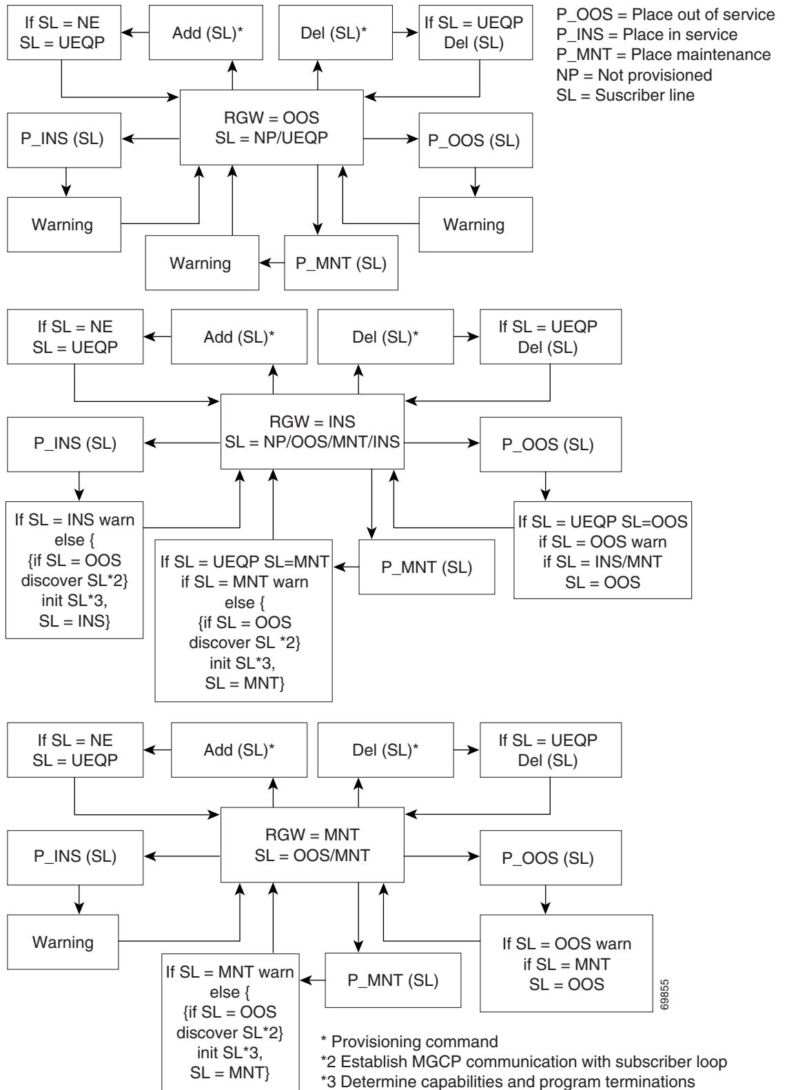
Figure 5-2 Administrative and Operational Maintenance States for Residential Gateways
