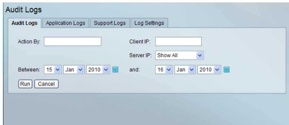
Figure 15-4 Audit Logs
