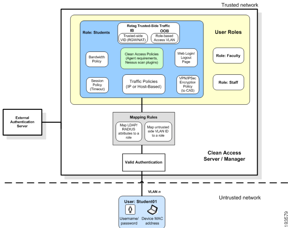
Figure 7-1 Normal Login User Roles
