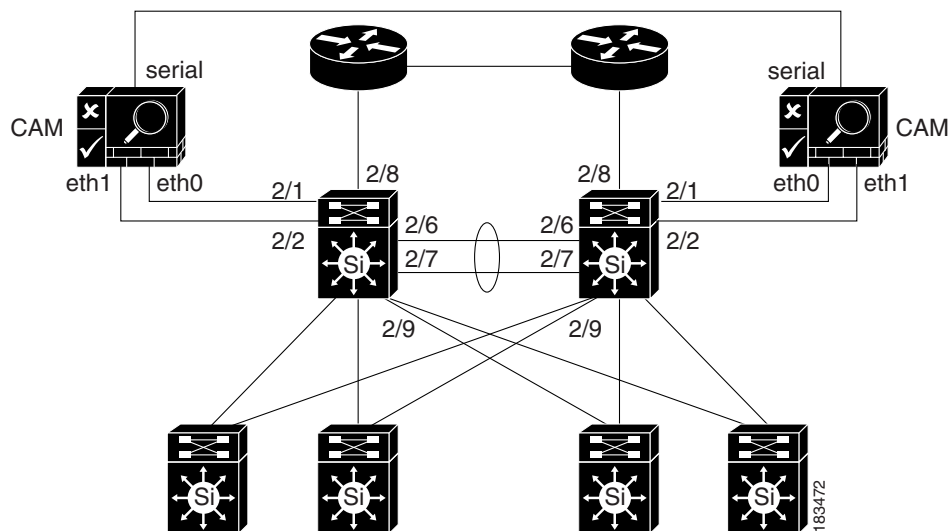
Figure 17-7 Adding HA CAMs to Network
