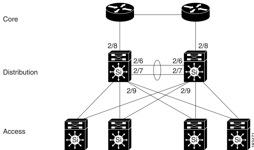
Figure 17-6 Example Core-Distribution-Access Network Before Cisco NAC Appliance
