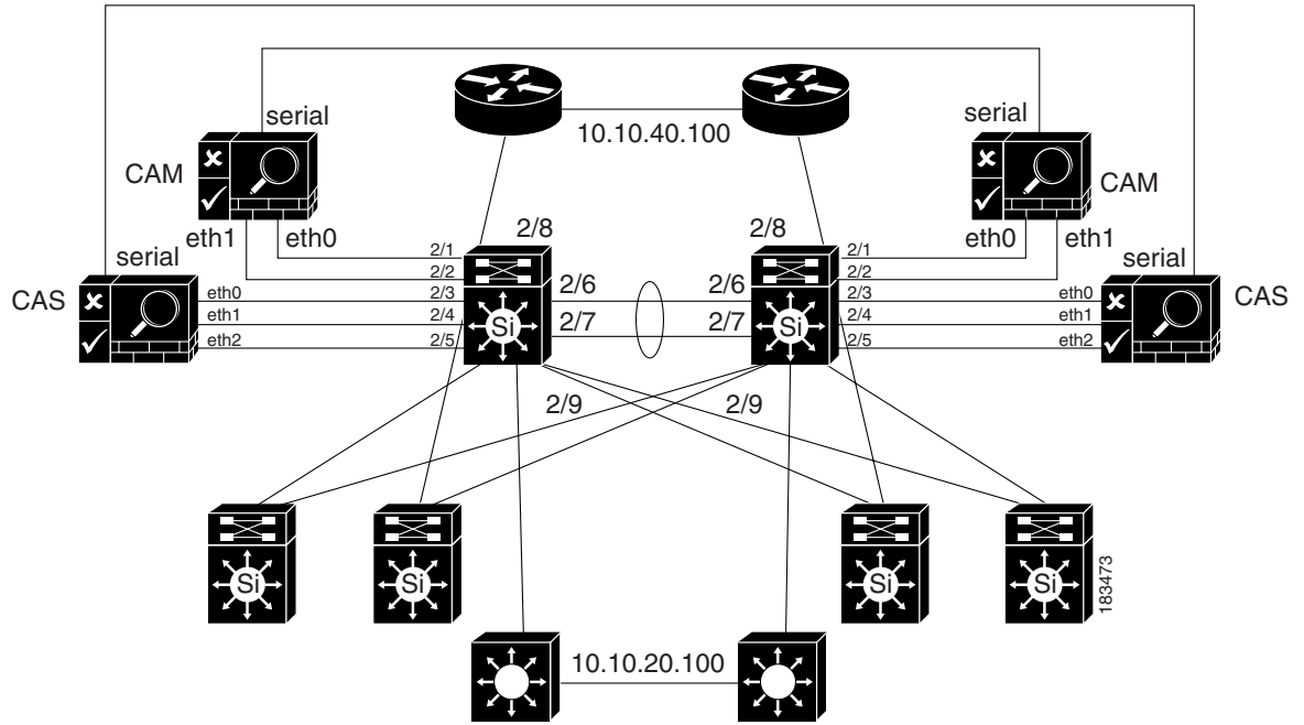
Figure 17-8 Adding HA CAS to Network
