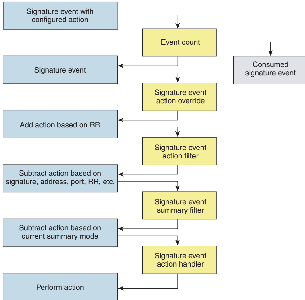
Figure 8-2 Signature Event Through the Signature Event Action Processor
