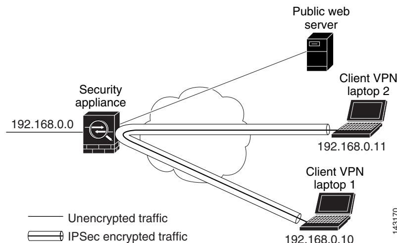
Figure 30-1 VPN Client Using Intra-Interface Feature for Hairpinning
