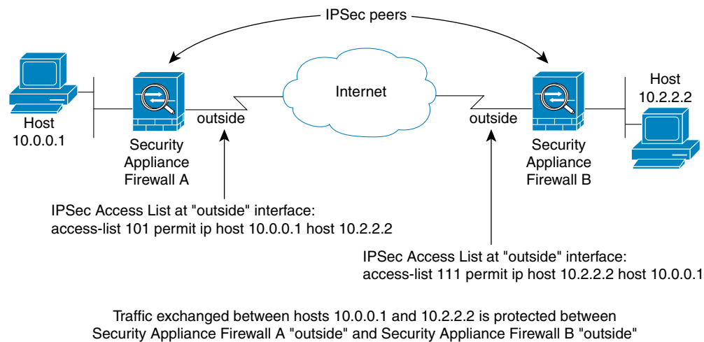
Figure 28-4 How Crypto Access Lists Apply to IPsec
