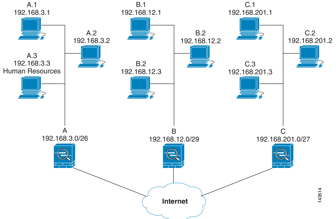
Figure 28-3 Effect of Permit and Deny ACEs on Traffic (Real Addresses)
