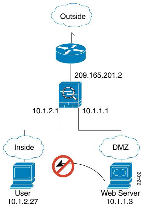
Figure 16-5 DMZ to Inside
