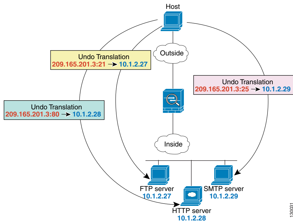
Figure 17-8 Static PAT
