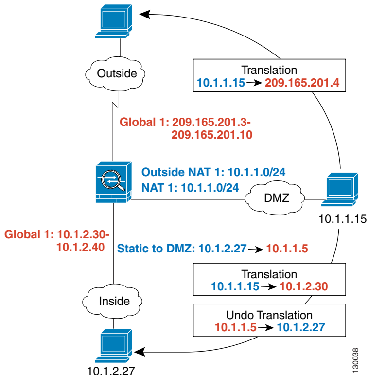
Figure 17-20 Outside NAT and Inside NAT Combined
