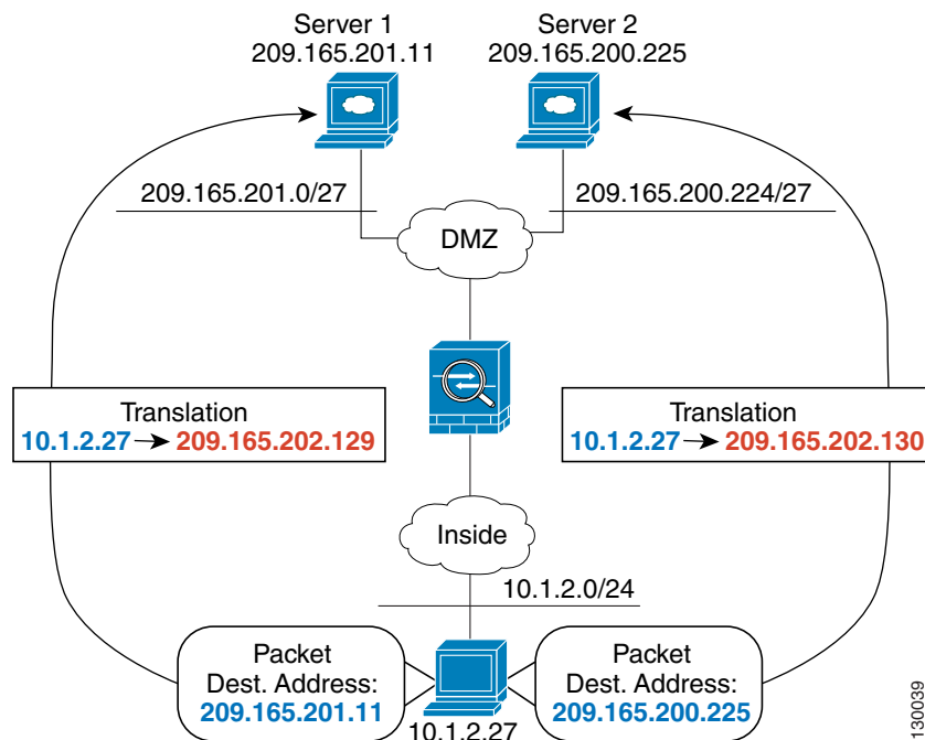
Figure 17-9 Policy NAT with Different Destination Addresses
