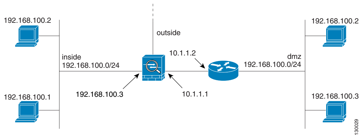
Figure 17-28 Using Outside NAT with Overlapping Networks
