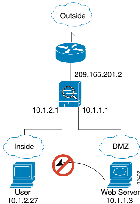
Figure 17-5 DMZ to Inside
