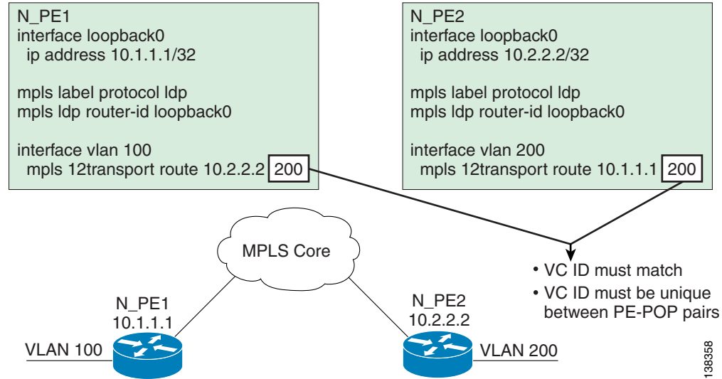
Figure D-4 Ethernet over MPLS Configuration
