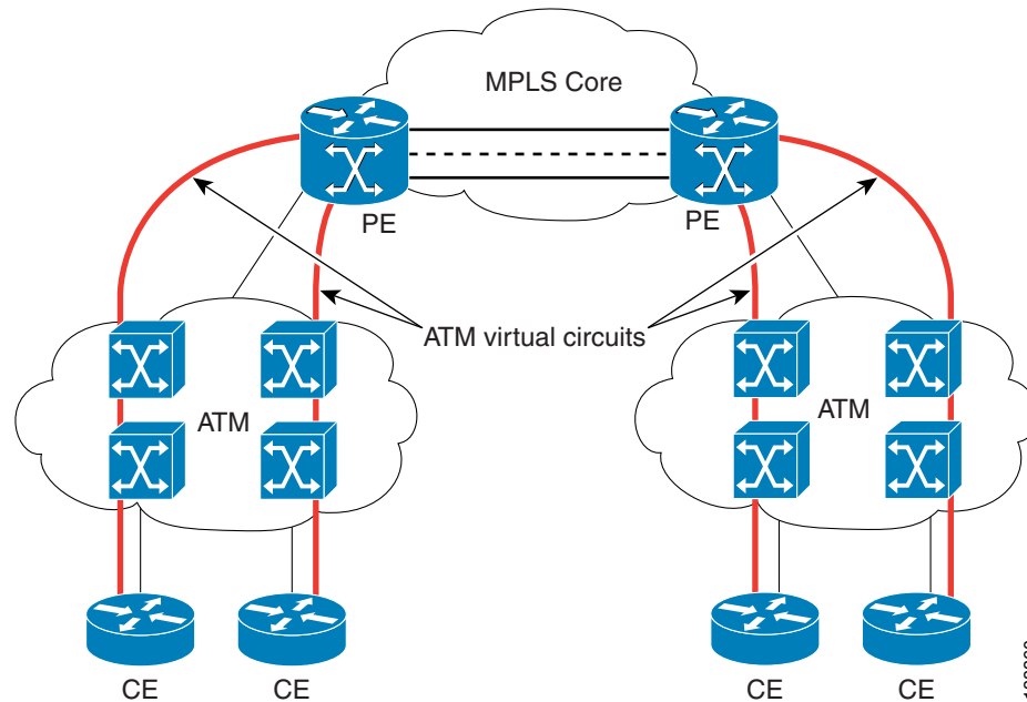
Figure D-7 Configuring AAL5 and Cell Relay over MPLS
