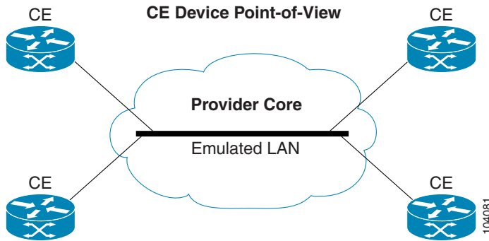
Figure D-9 MPLS-Based VPLS Topology
