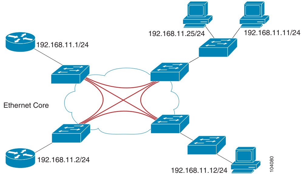
Figure D-11 VPLS EWS Topology
