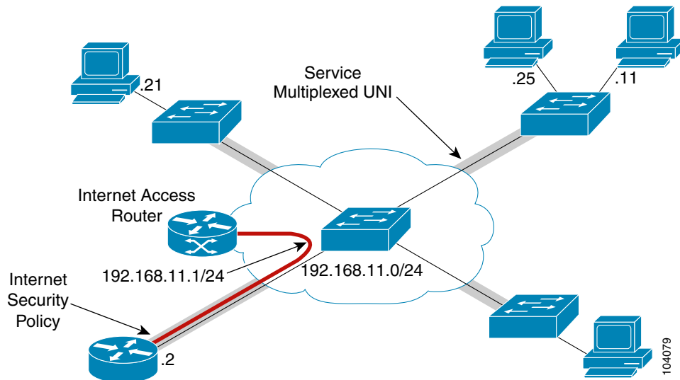
Figure D-12 VPLS ERS (EVP-LAN) Multipoint Topology
