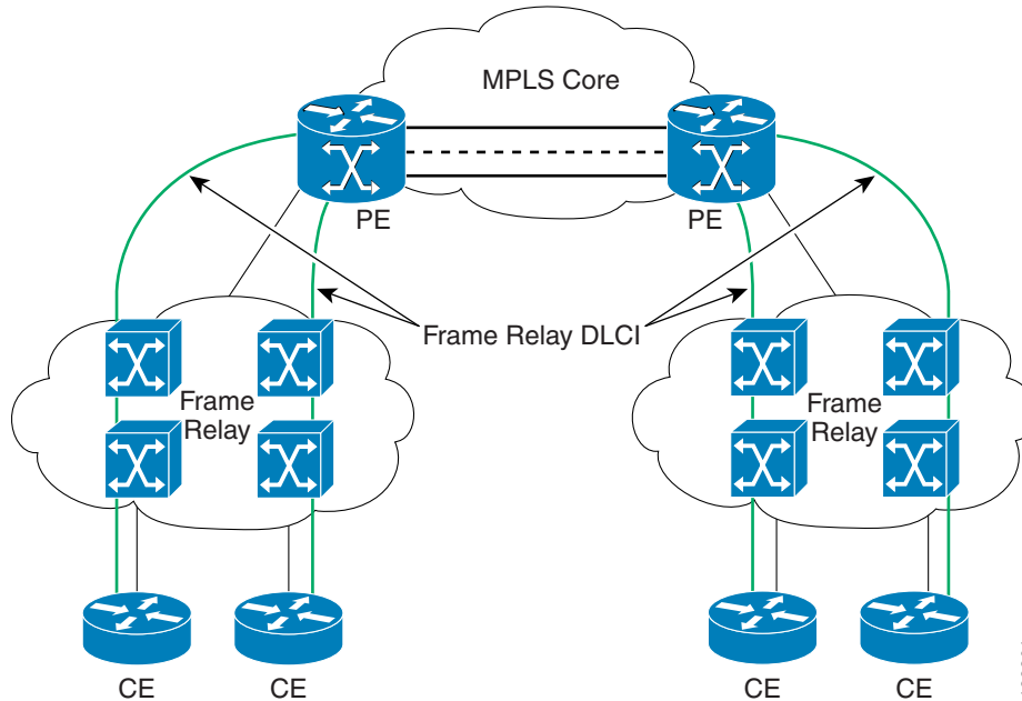
Figure D-8 Frame Relay over MPLS
