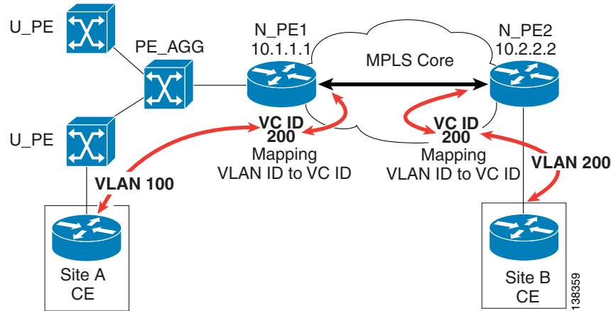
Figure D-6 VLAN-VC ID Mapping
