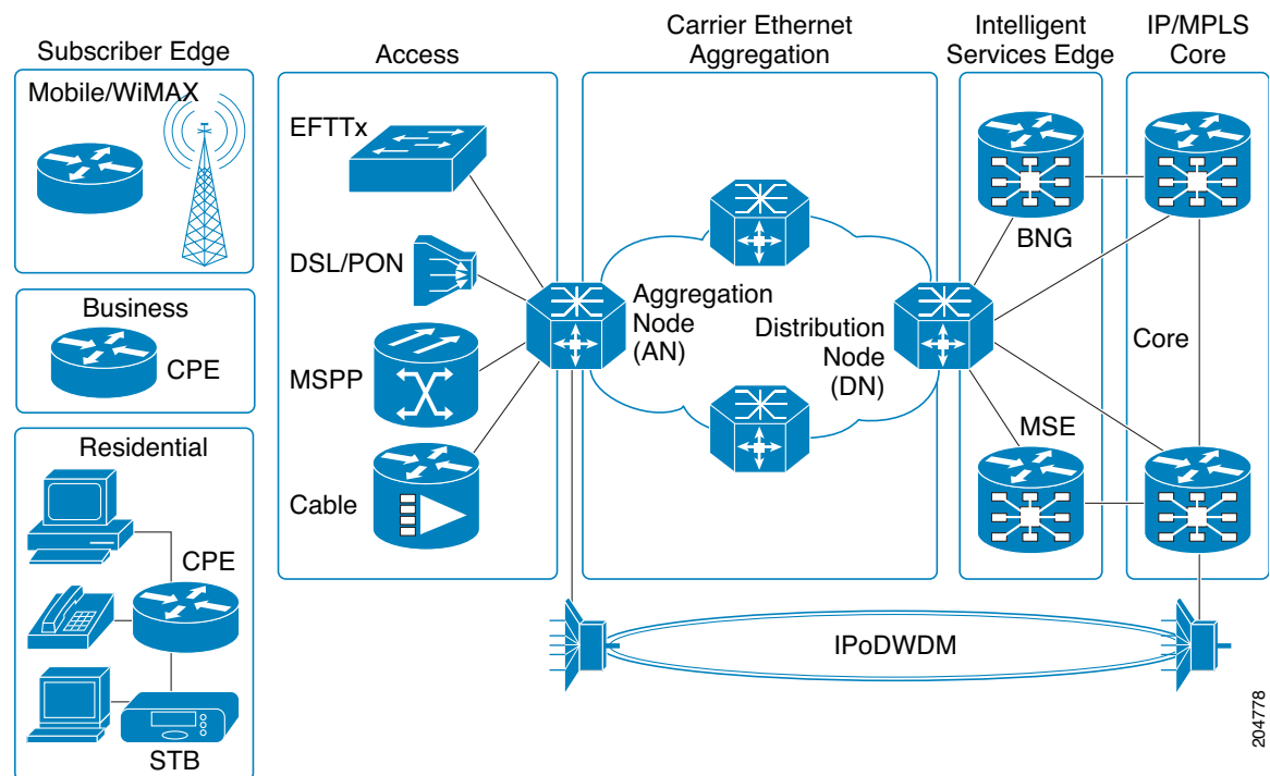
Figure D-1 IP NGN Carrier Ethernet Design
