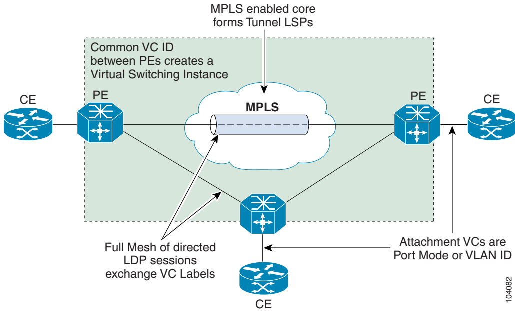
Figure D-10 Full Mesh of Emulated VCs
