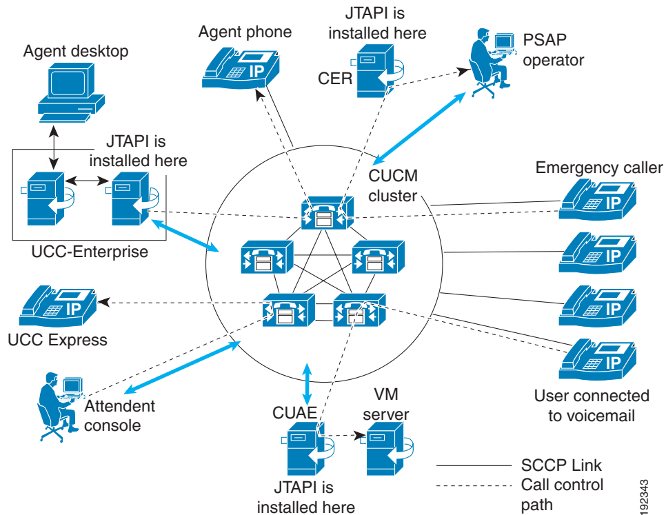
Figure 1-1 Cisco Unified Communications Manager and Cisco Unified JTAPI
