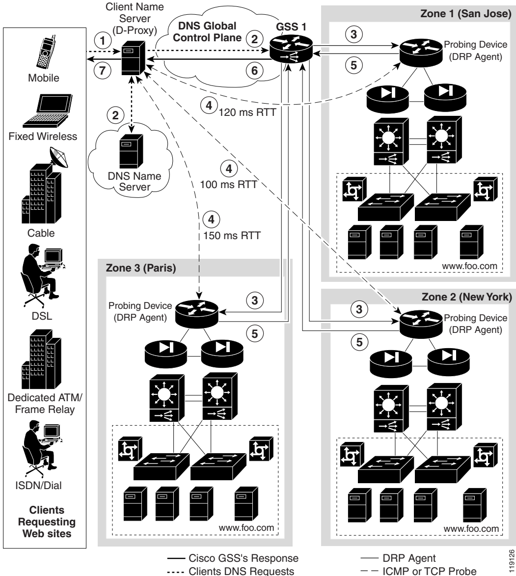
Figure 9-2 Network Proximity Using the Cisco Global Site Selector
