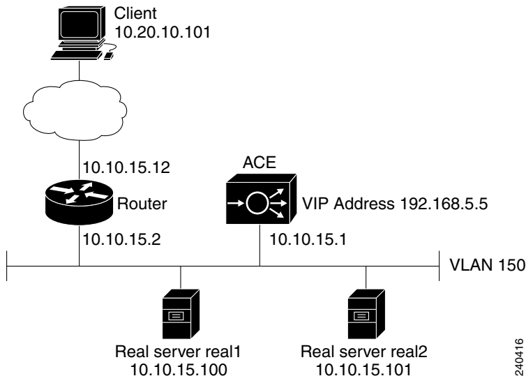
Figure 2-1 ASN Network Topology Example
