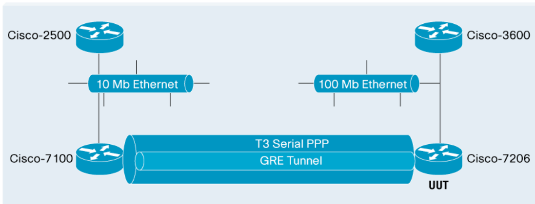
Figure 20. GRE Testbed
