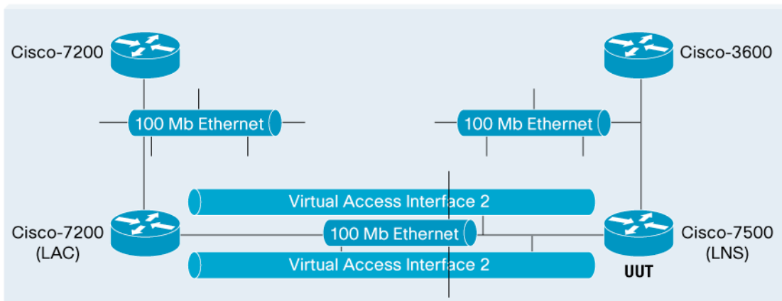
Figure 26. L2TP Testbed
