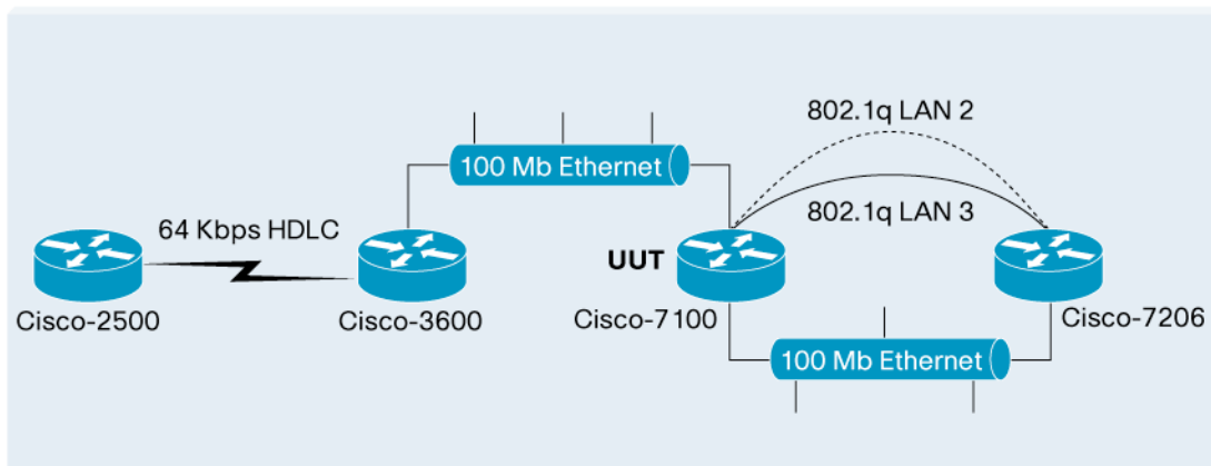
Figure 14. 802.1q Testbed
