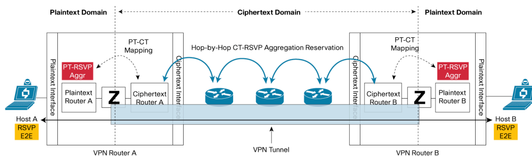
Figure 10. Possible Solution Architecture
