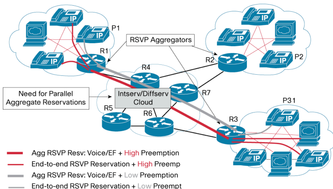
Figure 8. Generic Aggregate RSVP Reservation
