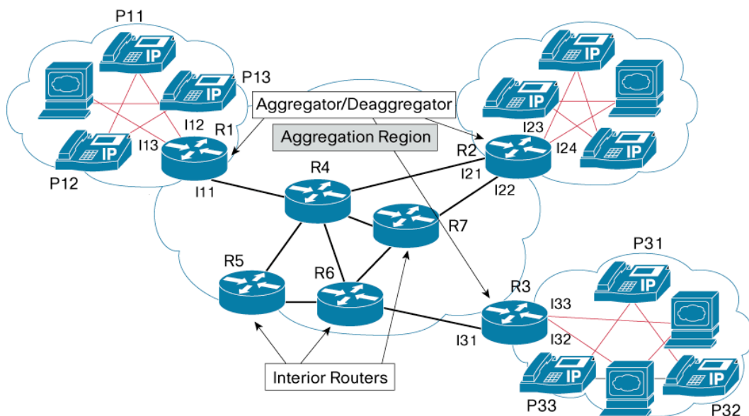
Figure 5. RSVP Aggregation Mechanism
