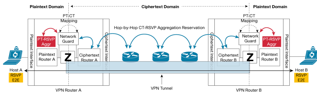
Figure 11. Solution Architecture with Network Guard
