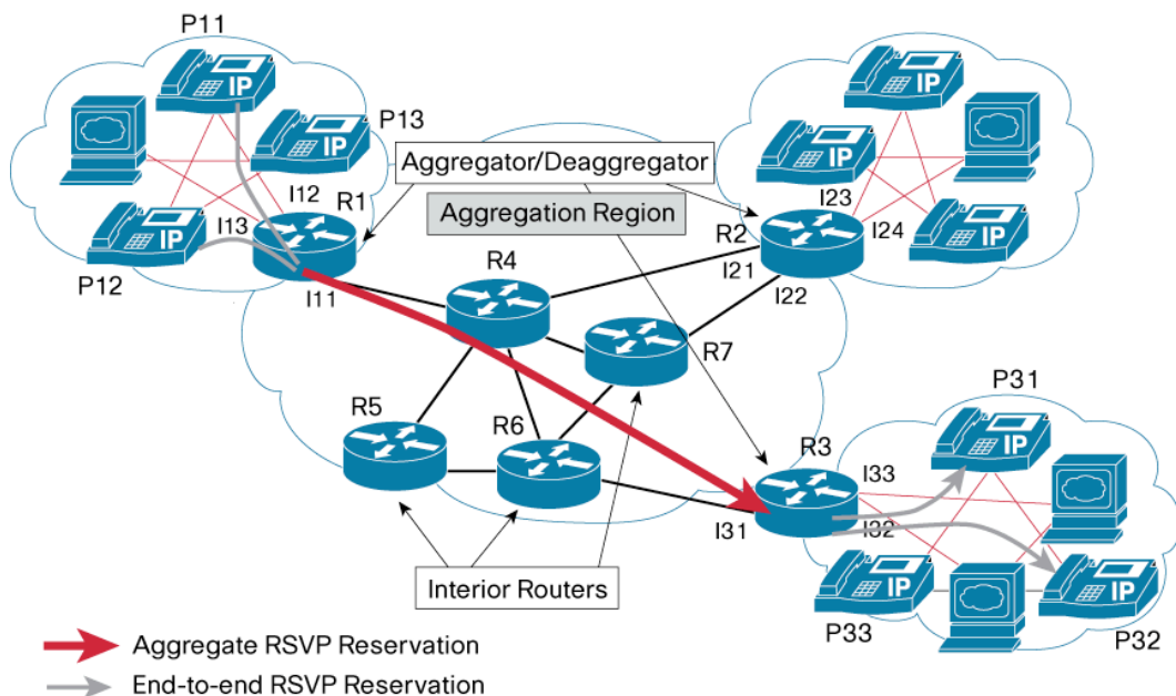
Figure 6. End Result of RSVP Aggregation Process
