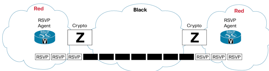
Figure 2. RSVP Deployment Issue in Multiple Security Domains Network
