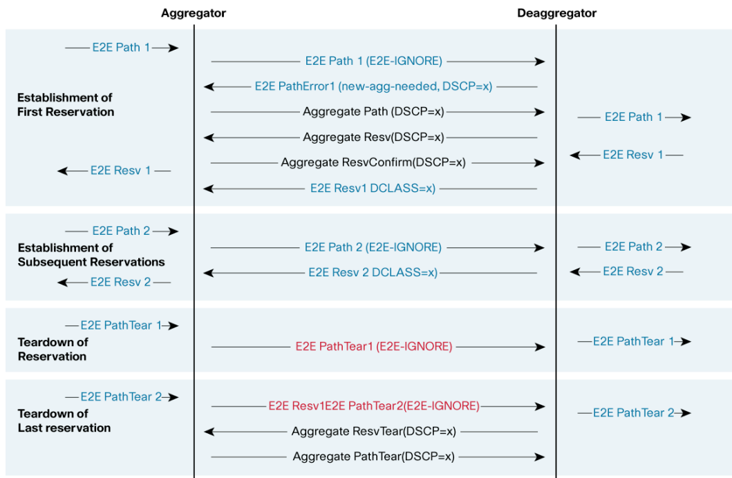
Figure 7. RSVP Aggregation Detailed Call Flow
