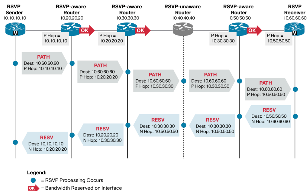
Figure 1. End-to-End RSVP Reservation
