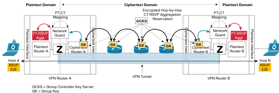
Figure 14. Solution Architecture with GDOI
