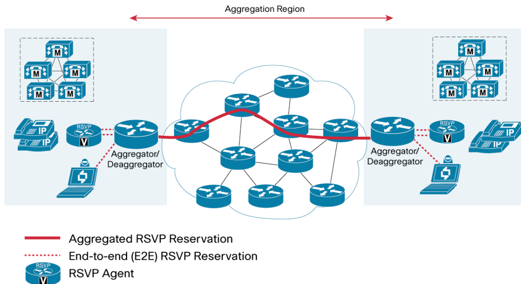
Figure 4. RSVP Aggregation Overview
