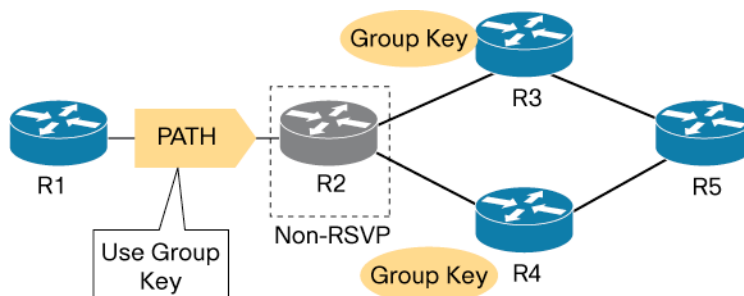
Figure 13. RSVP Encryption with Group Keying
