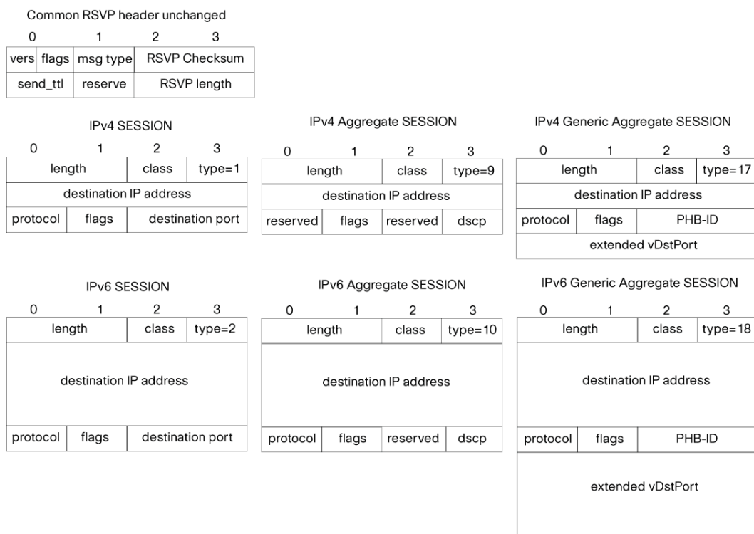
Figure 9. Message Format for RSVP Aggregation
