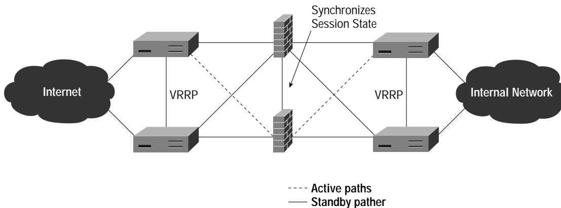
Figure 4 Fully Redundant Firewall Load-Balancing Example
