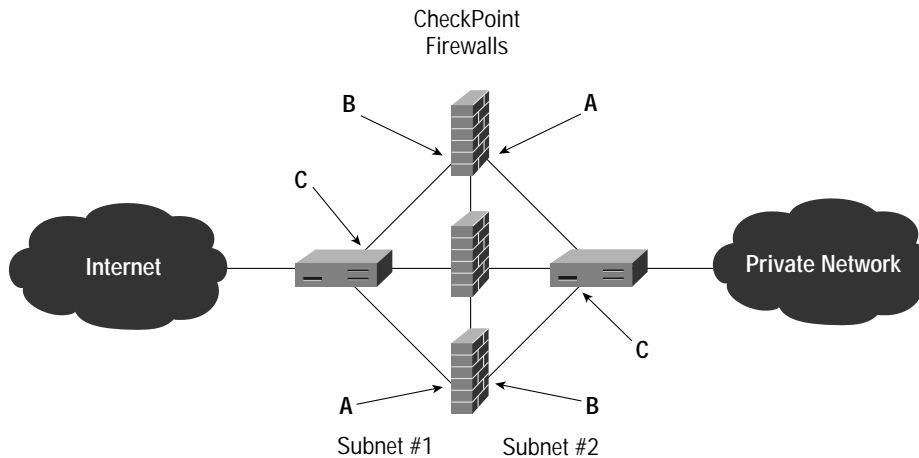
Figure 3 Load-Balanced Firewall Configuration
