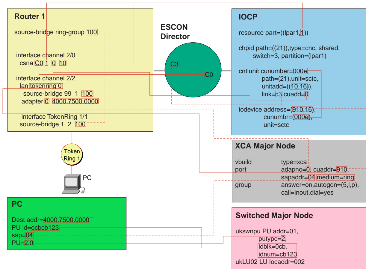
Figure 2 CSNA Parameter Relationships
