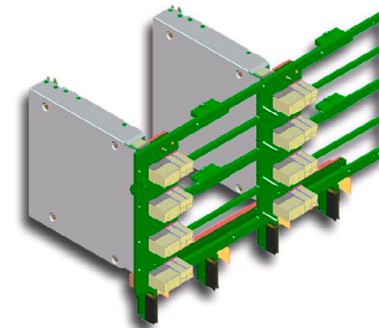
Figure 6: Cisco UCS 5108 Blade Server Chassis Open Midplane Design Increases Airflow Efficiency
