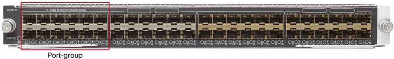
Figure 1. Port Group on a 48-port 1/21/2/4 Gbps Linecard Module
