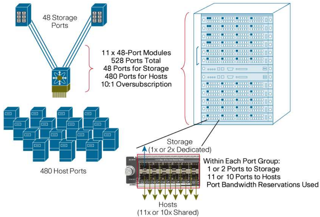
Figure 3. 528-Port Collapsed Core SAN Design
