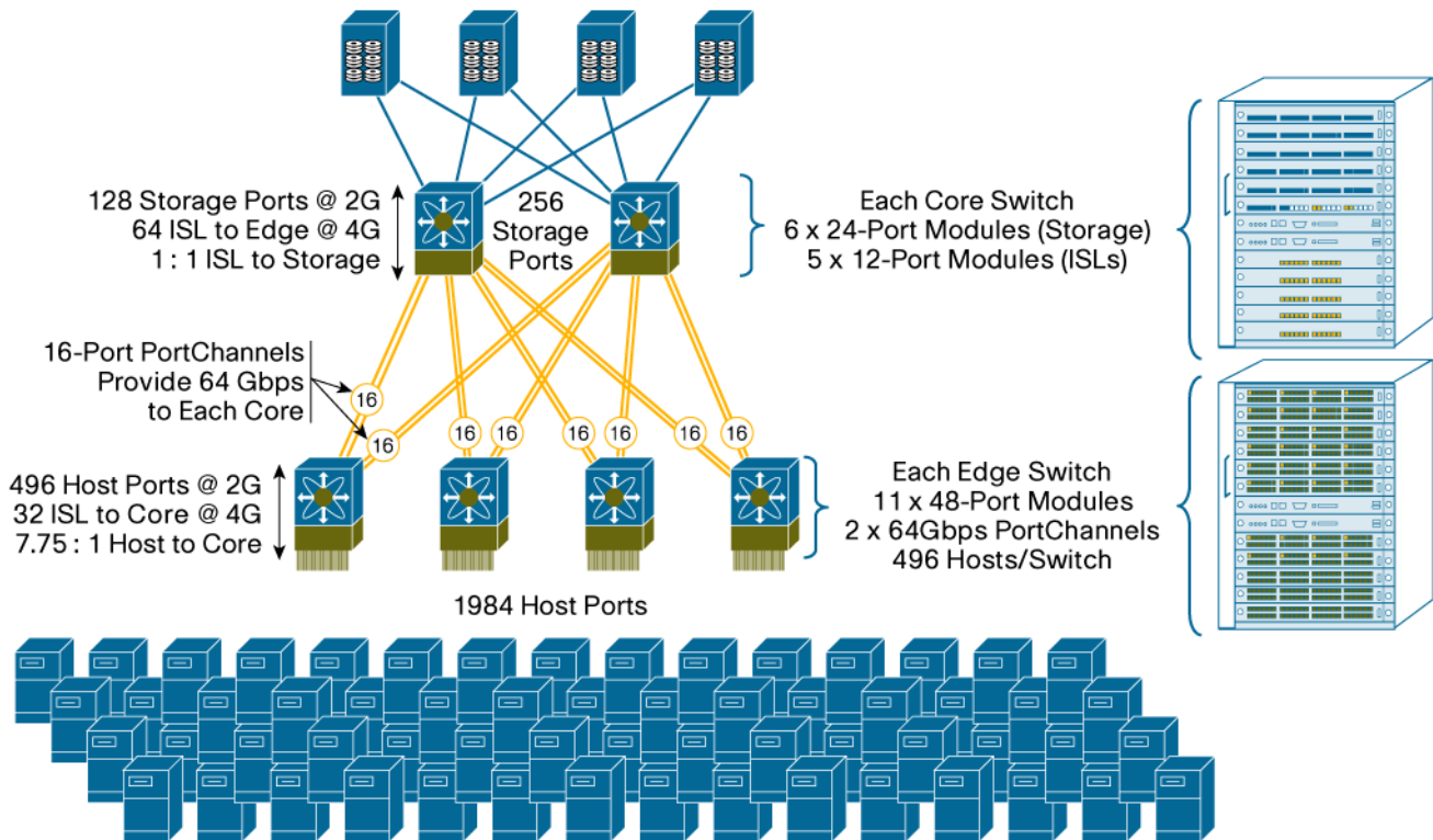
Figure 4. 2240-Port Core/Edge SAN Design
