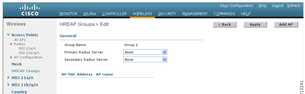
Figure 12-11 HREAP Groups > Edit Page
