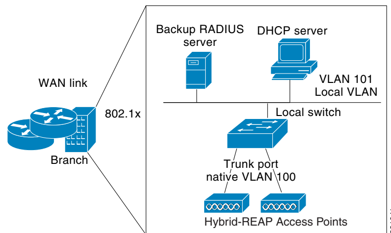
Figure 12-9 Hybrid-REAP Group Deployment
