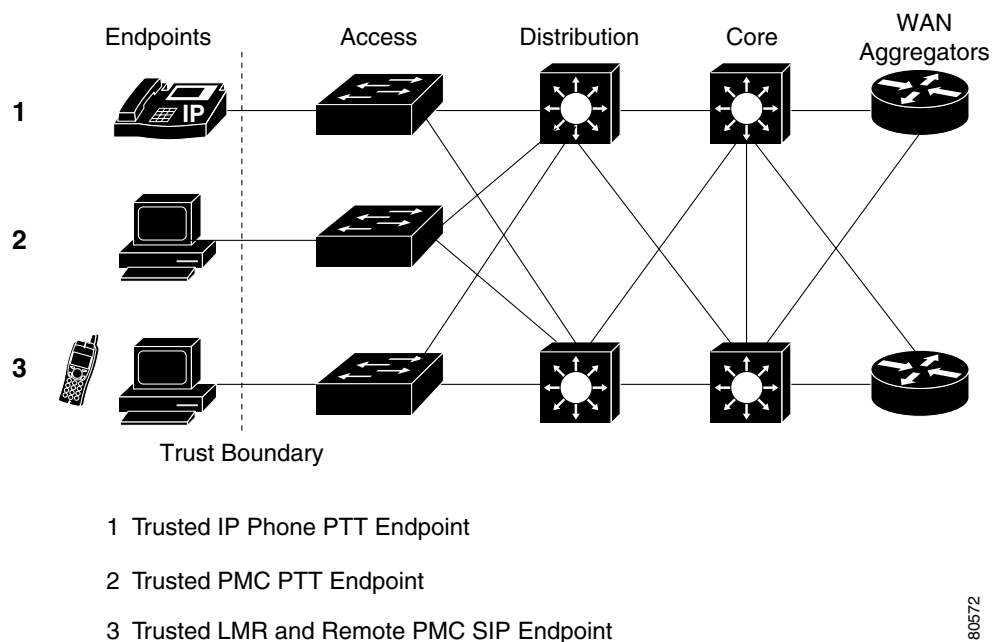
Figure 4-4 Trust Boundary
