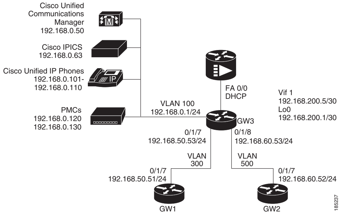
Figure 4-2 Redundant RMS Core Topology
