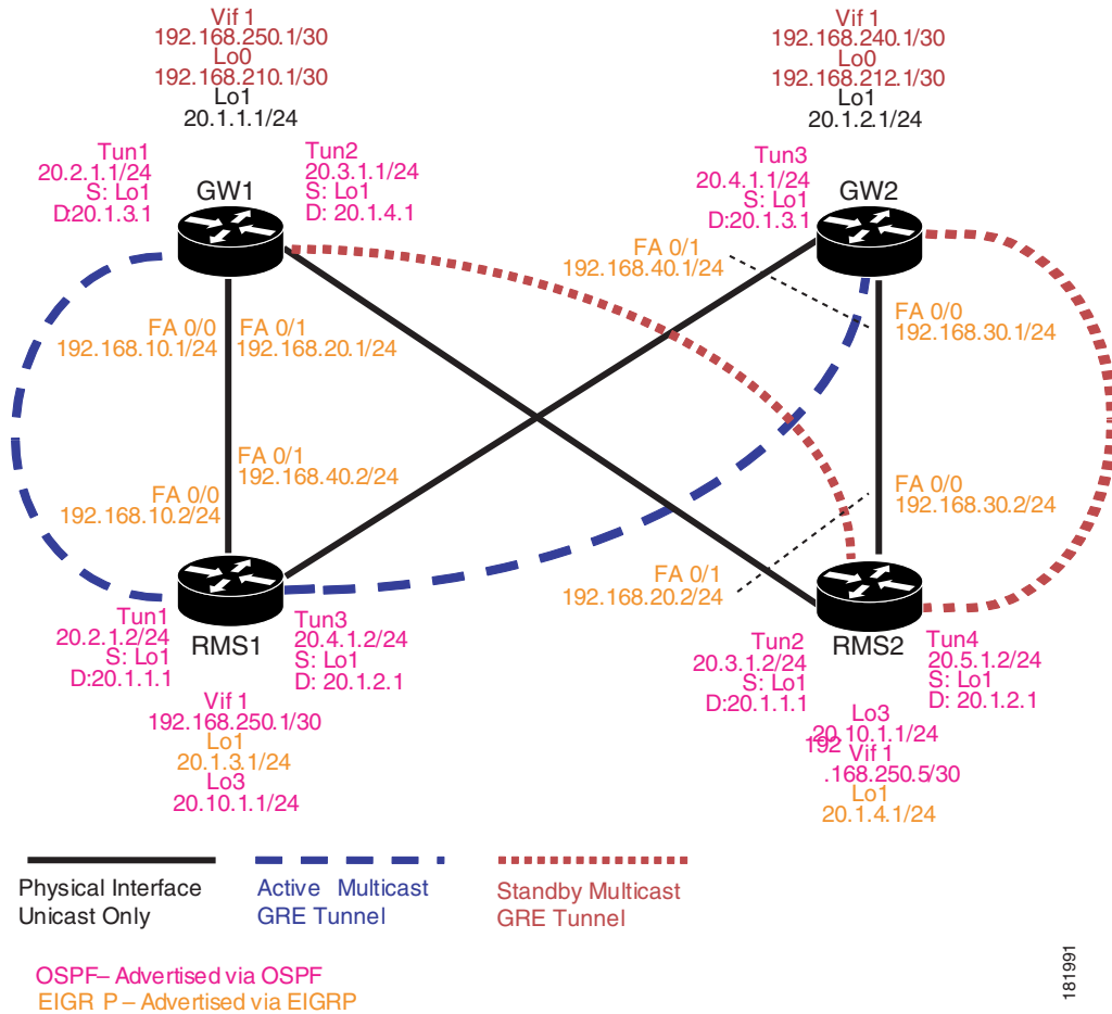
Figure 4-3 Router Interfaces to Core
