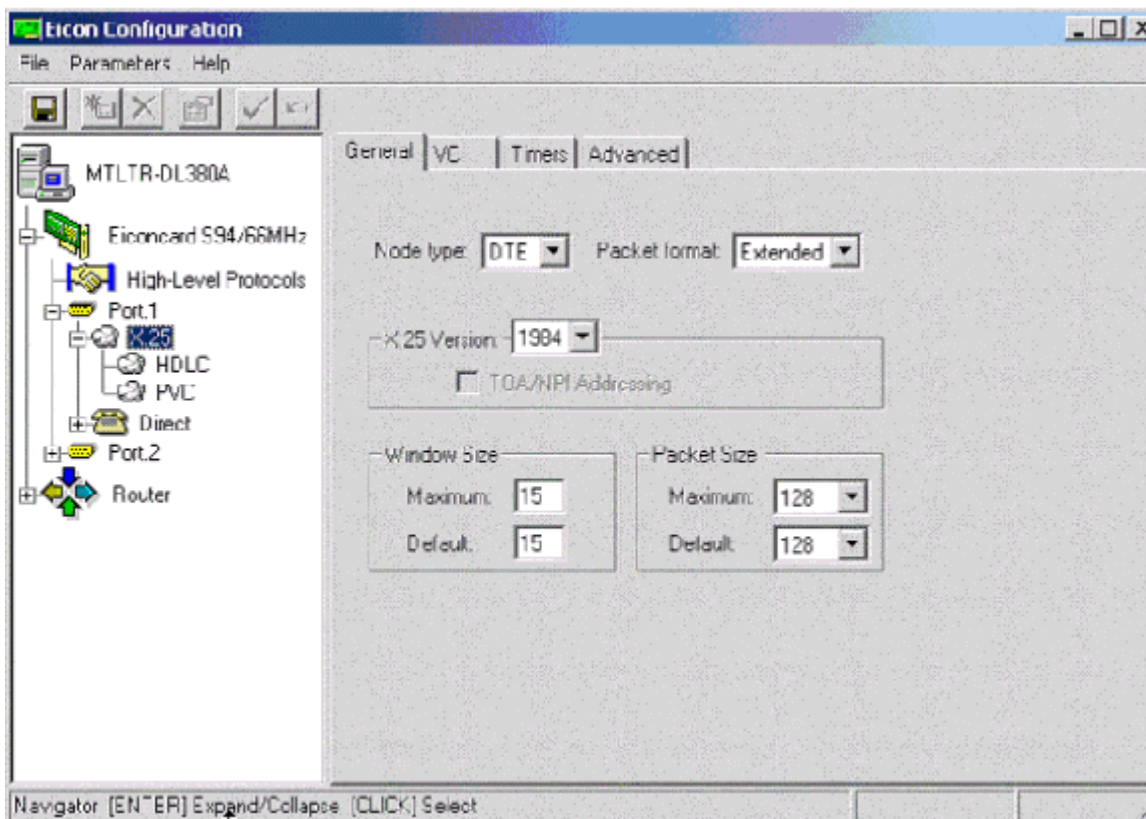
Figure 5: X.25 Packet-Level Protocol—General Configuration
