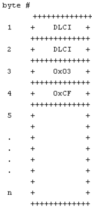
Figure 4. MLPoFR Header
