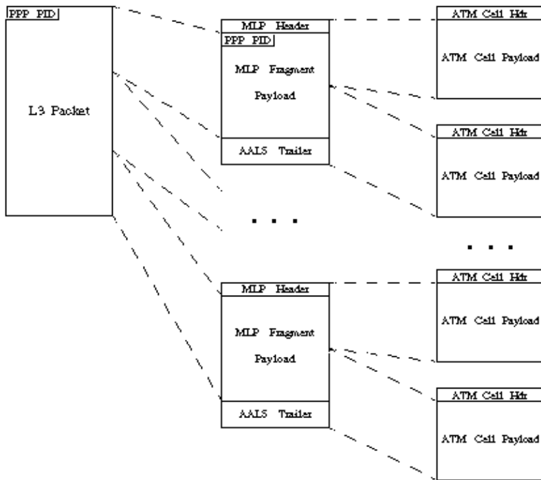
Figure 3. How the MLPPPoATM packet is fragmented using VC Multiplexing.
