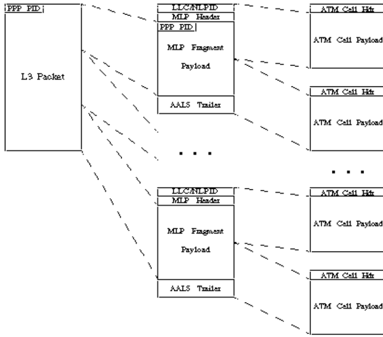
Figure 2. How the MLPPPoATM packet is fragmented using NLPID.
