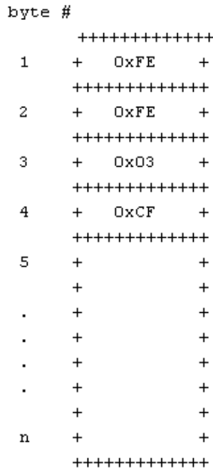
Figure 5. MLPoATM Header
