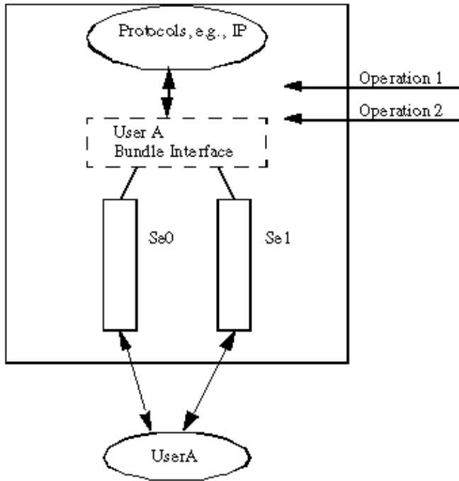
Figure 2. Multilink PPP Bundle Interface
