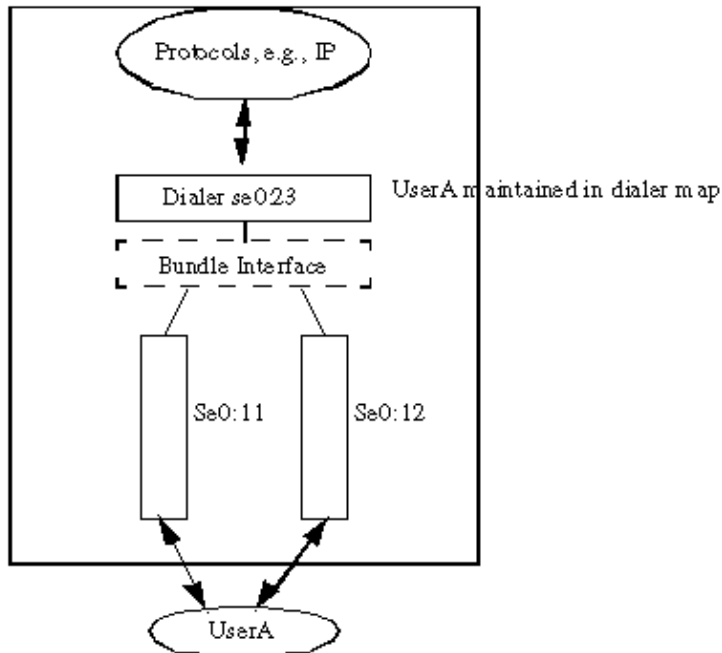
Figure 3. Multilink PPP Interface (Passive)
