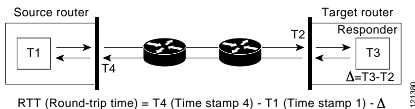
Figure 41-2 Cisco IOS IP SLAs Responder Time Stamping
