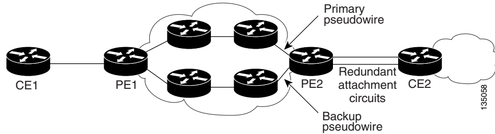
Figure 6-3 Pseudowire Redundancy
