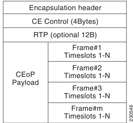
Figure 6-2 Structured Mode Frame Format
