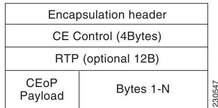
Figure 6-1 Unstructured Mode Frame Format
