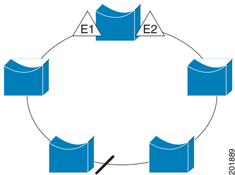
Figure 17-2 REP Ring Segment
