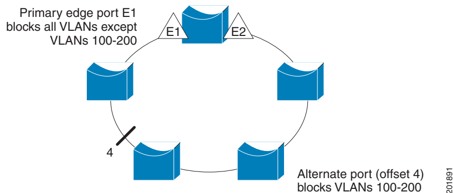
Figure 17-5 Example of VLAN Blocking
