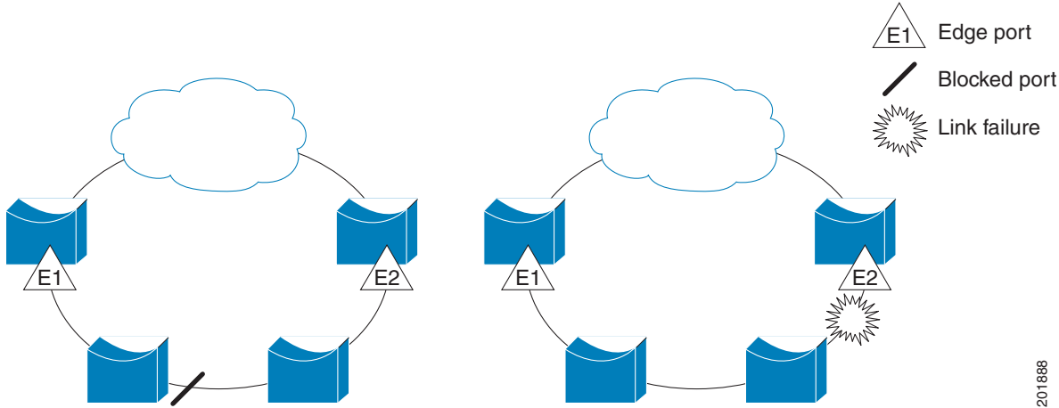
Figure 17-1 REP Open Segments
