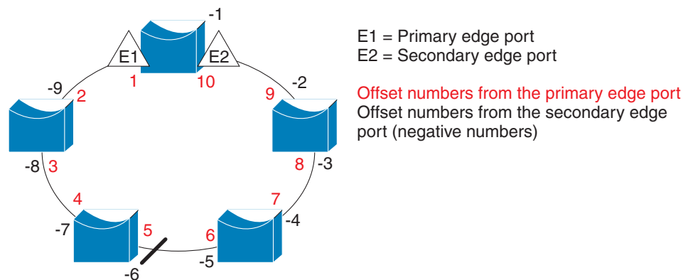
Figure 17-4 Neighbor Offset Numbers in a Segment
