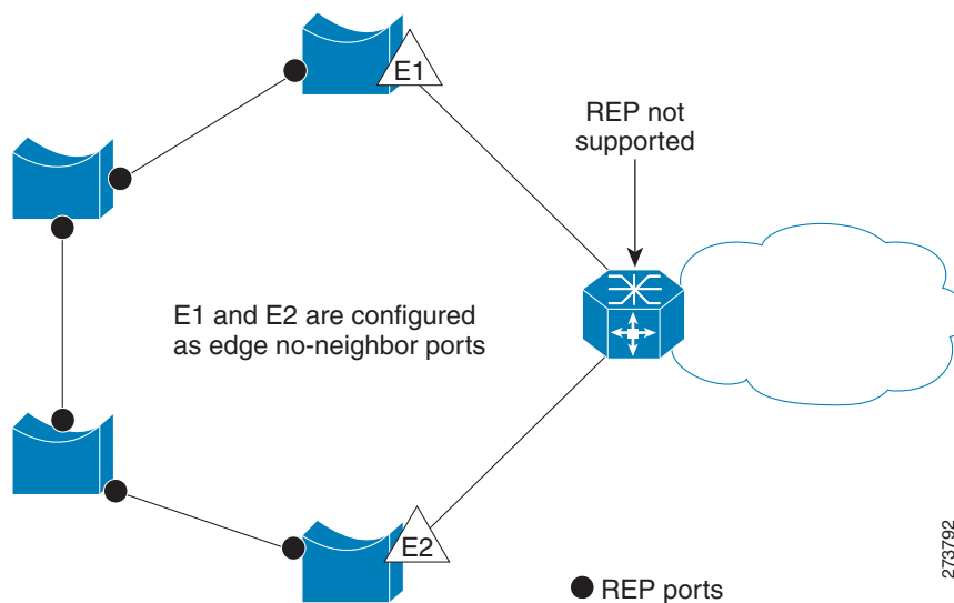
Figure 17-3 Edge No-Neighbor Ports
