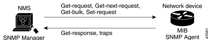
Figure 27-1 SNMP Network
