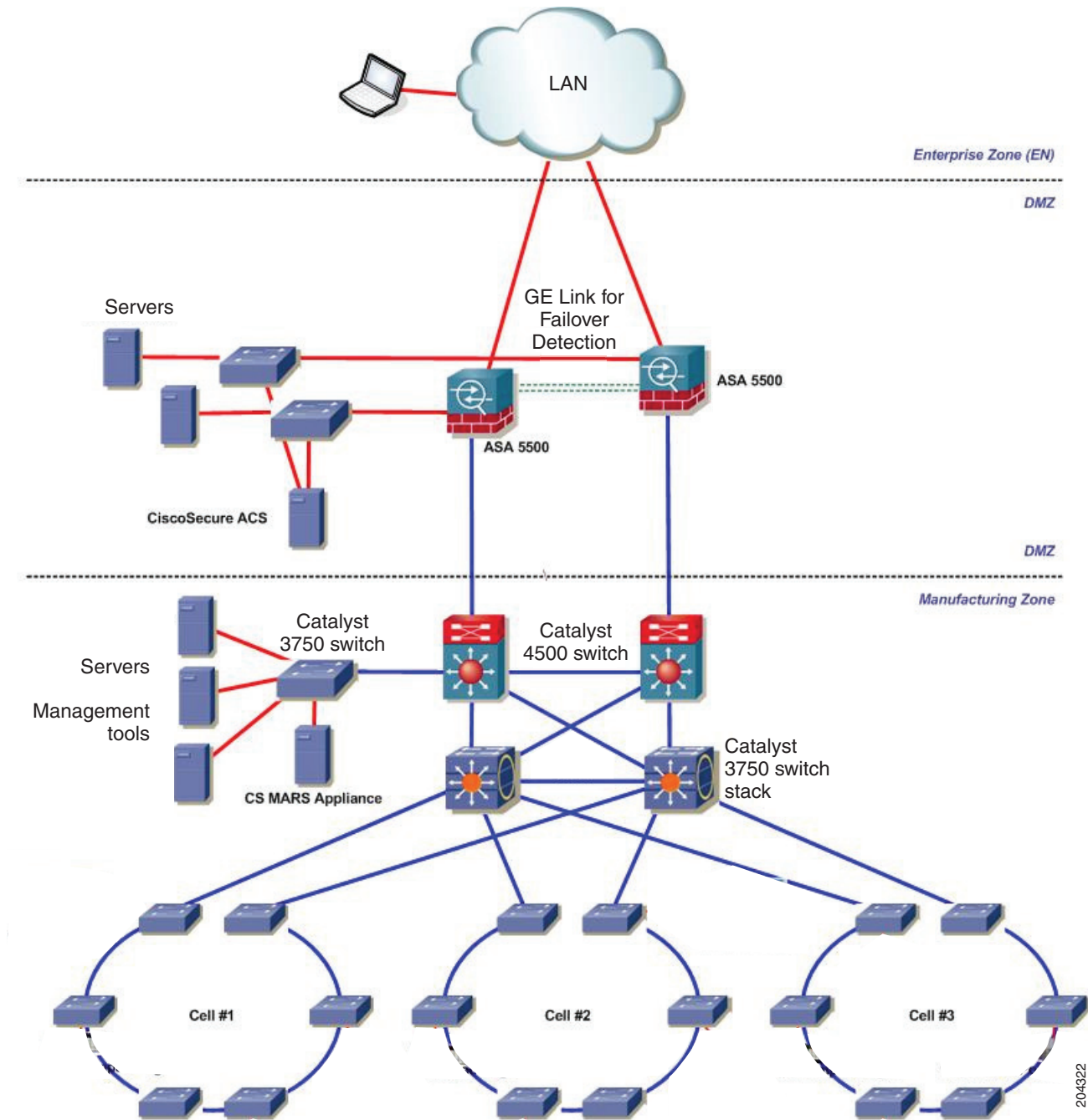
Figure 1-1 Ethernet-to-the-Factory Architecture
