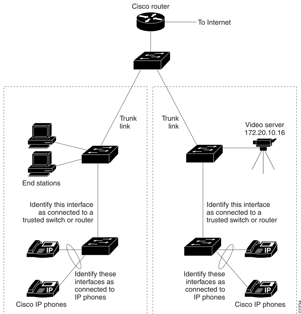
Figure 40-1 Auto-QoS Configuration Example Network
