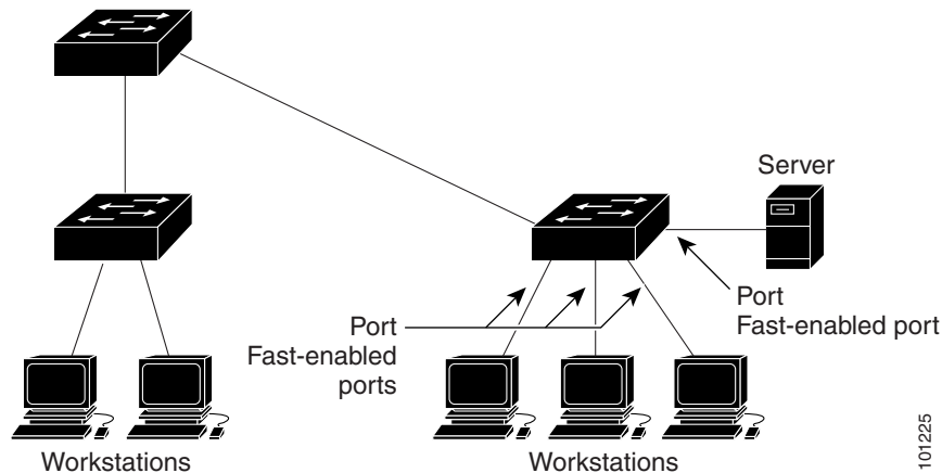
Figure 23-1 PortFast-Enabled Interfaces
