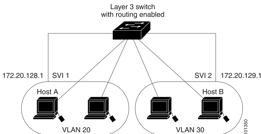
Figure 16-1 Connecting VLANs with a Layer 3 Switch
