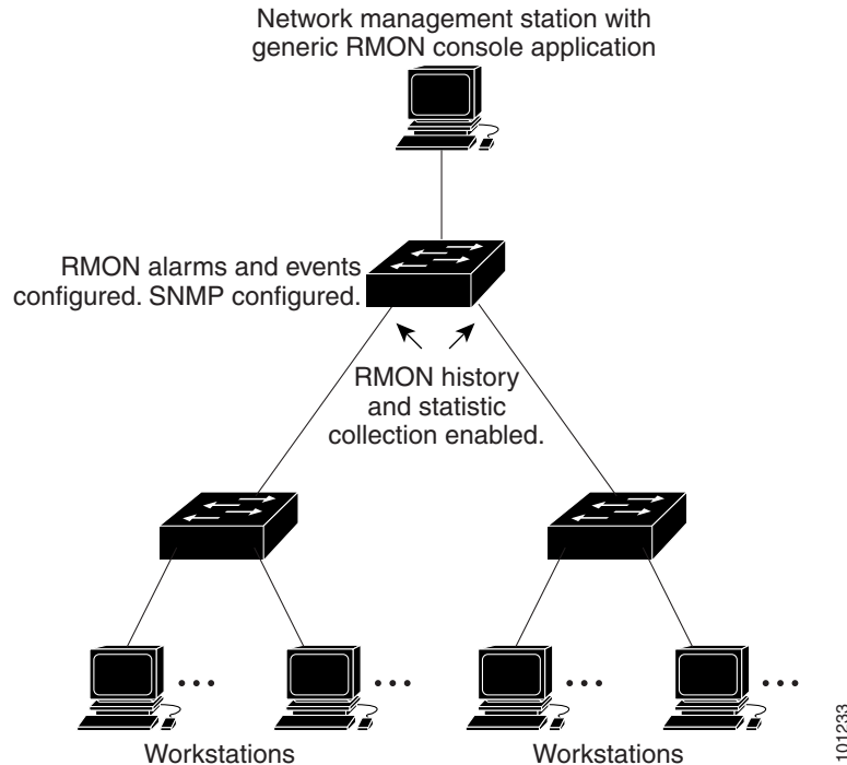
Figure 35-1 Remote Monitoring Example
