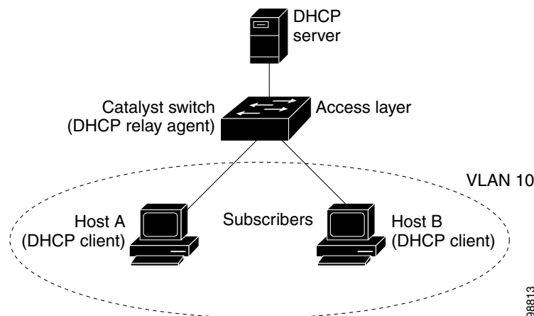
Figure 26-1 DHCP Relay Agent in a Metropolitan Ethernet Network
