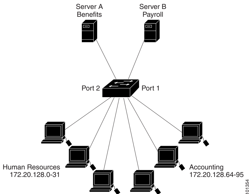
Figure 38-2 Using Router ACLs to Control Traffic
