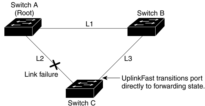
Figure 23-4 UplinkFast Example After Direct Link Failure
