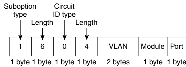
Figure 26-2 Suboption Packet Formats
