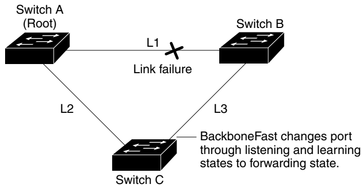
Figure 23-6 BackboneFast Example After Indirect Link Failure
