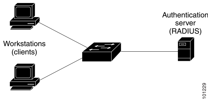
Figure 13-5 Multiple Host Mode Example
