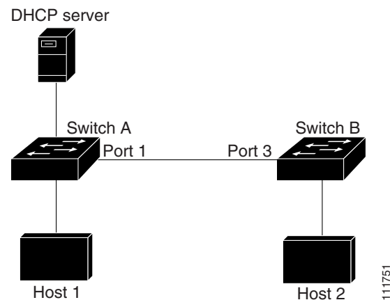
Figure 27-2 ARP Packet Validation on a VLAN Enabled for DAI
