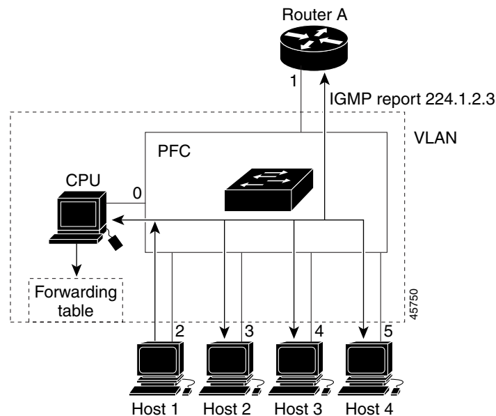
Figure 29-1 Initial IGMP Join Message
