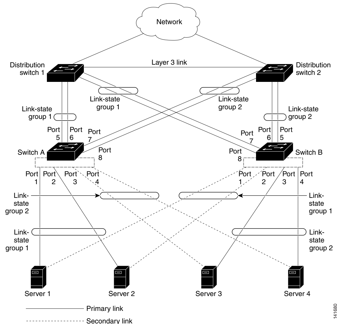
Figure 44-1 Typical Link State Tracking Configuration
