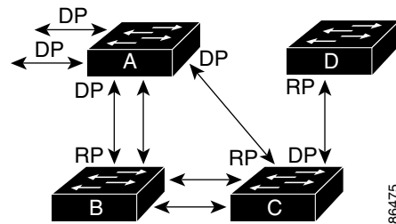
Figure 21-2 Spanning-Tree Topology
