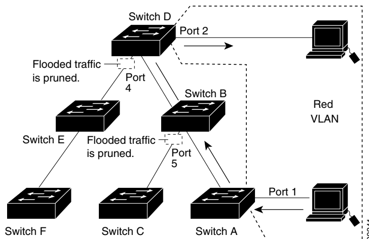
Figure 19-2 Optimized Flooded Traffic with VTP Pruning
