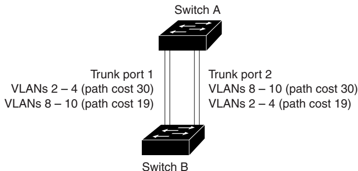
Figure 18-3 Load-Sharing Trunks with Traffic Distributed by Path Cost
