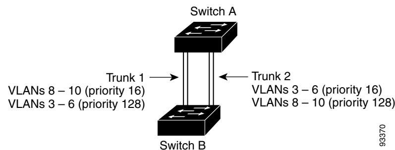
Figure 18-2 Load Sharing by Using STP Port Priorities
