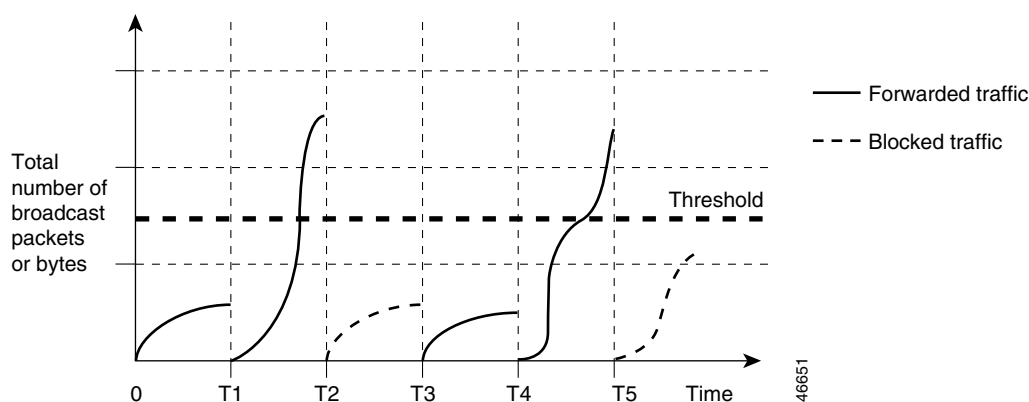
Figure 30-1 Broadcast Storm Control Example
