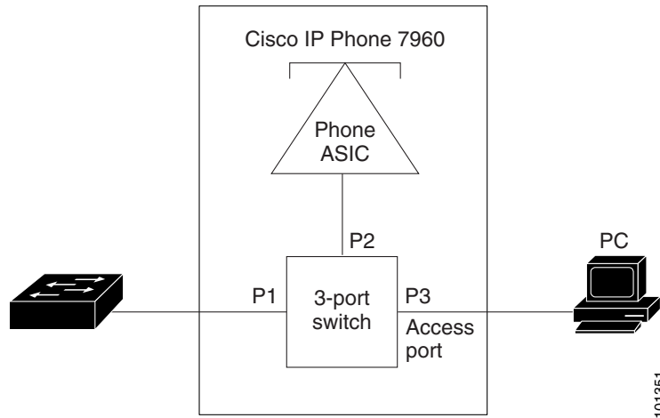
Figure 20-1 Cisco 7960 IP Phone Connected to a Switch
