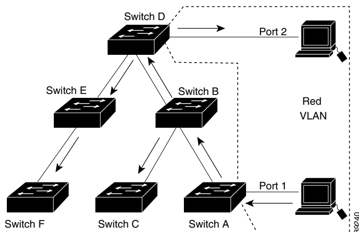
Figure 19-1 Flooding Traffic without VTP Pruning
