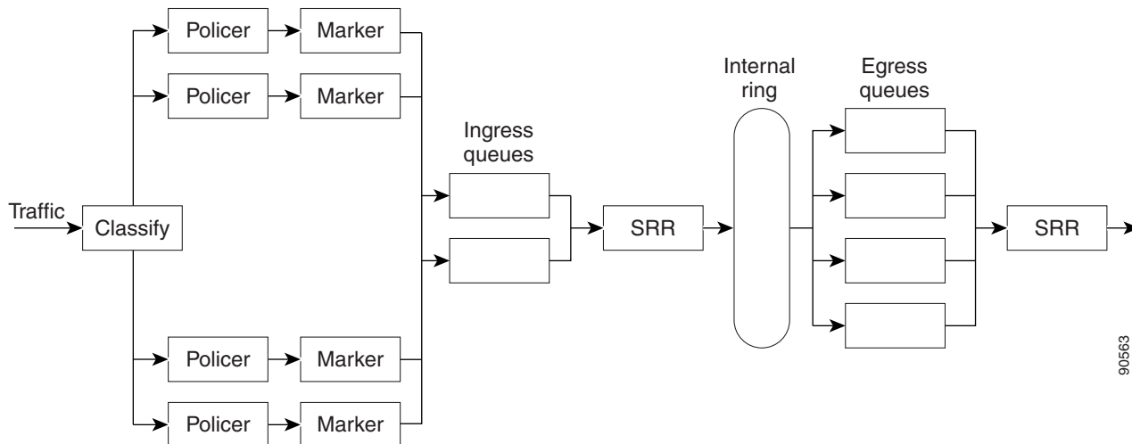
Figure 36-7 Ingress and Egress Queue Location on Catalyst 3560-E Switches
