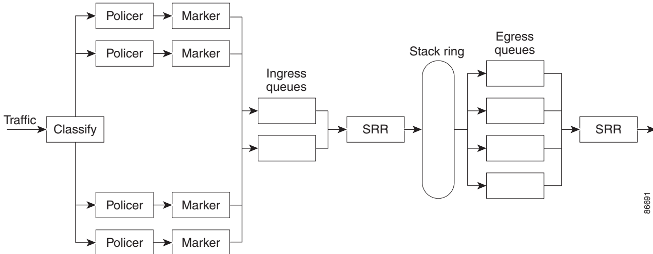
Figure 36-6 Ingress and Egress Queue Location on Catalyst 3750-E Switches
