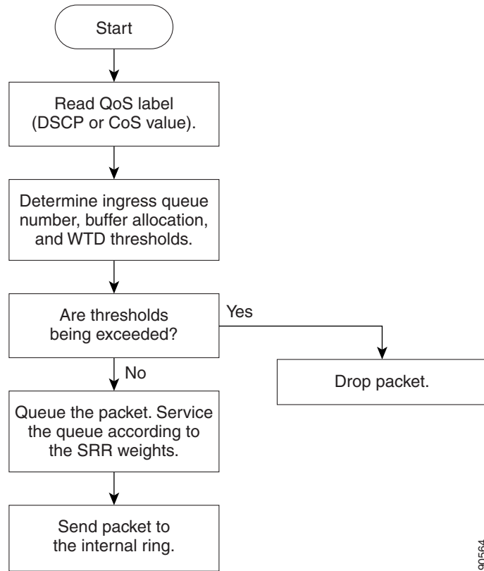
Figure 36-10 Queueing and Scheduling Flowchart for Ingress Ports on Catalyst 3560-E Switches
