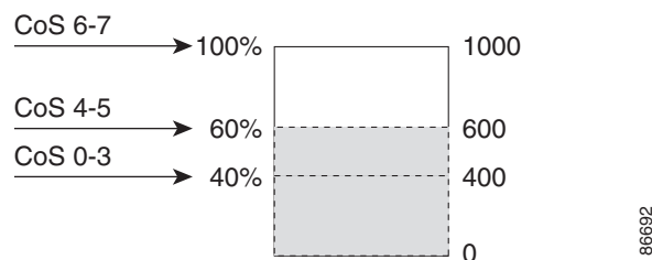
Figure 36-8 WTD and Queue Operation
