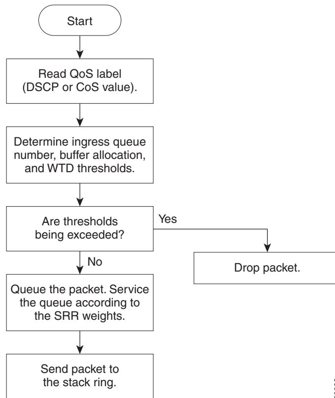
Figure 36-9 Queueing and Scheduling Flowchart for Ingress Ports on Catalyst 3750-E Switches
