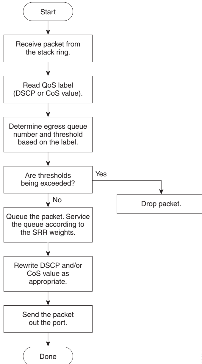
Figure 36-11 Queueing and Scheduling Flowchart for Egress Ports on Catalyst 3750-E Switches
