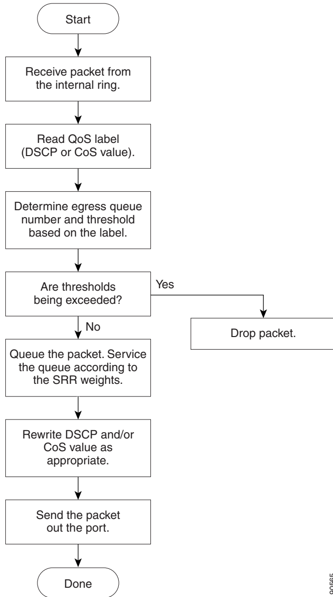
Figure 36-12 Queuing and Scheduling Flowchart for Egress Ports on Catalyst 3560-E Switches
