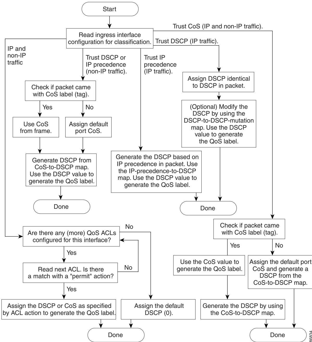
Figure 36-3 Classification Flowchart
