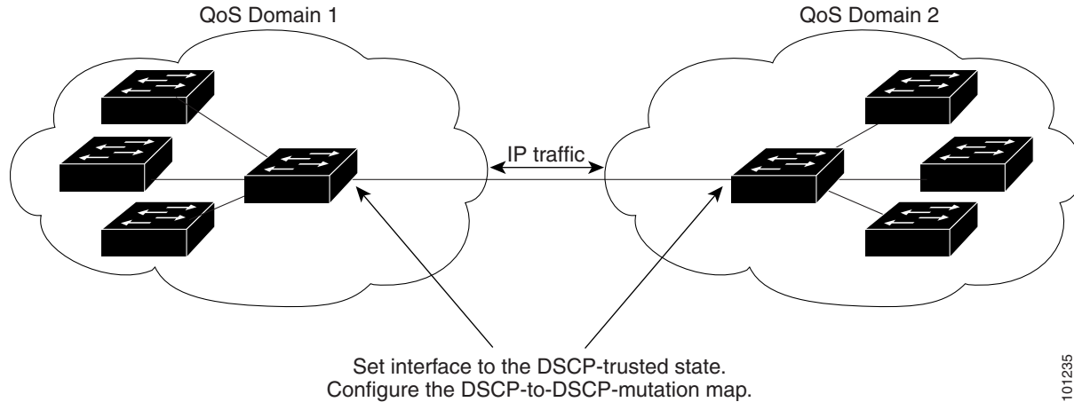
Figure 36-15 DSCP-Trusted State on a Port Bordering Another QoS Domain
