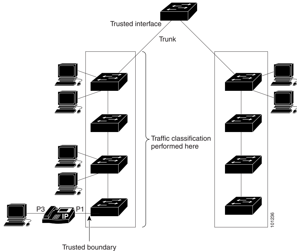
Figure 36-14 Port Trusted States within the QoS Domain
