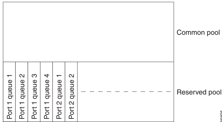
Figure 36-13 Egress Queue Buffer Allocation
