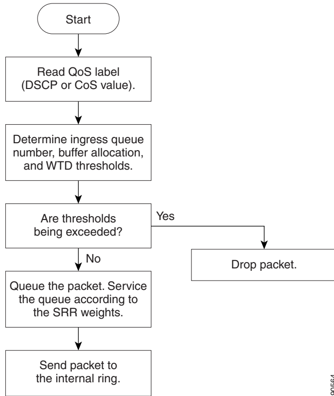
Figure 38-10 Queuing and Scheduling Flowchart for Ingress Ports on Catalyst 3560-E Switches
