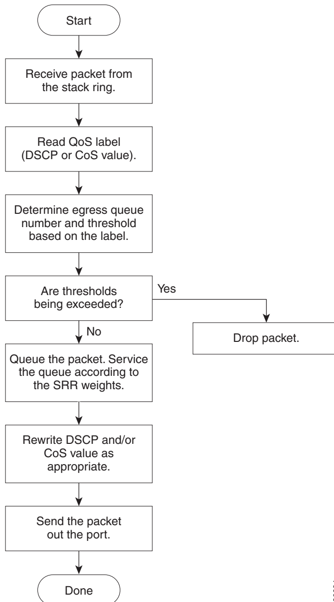
Figure 38-11 Queueing and Scheduling Flowchart for Egress Ports on Catalyst 3750-E Switches
