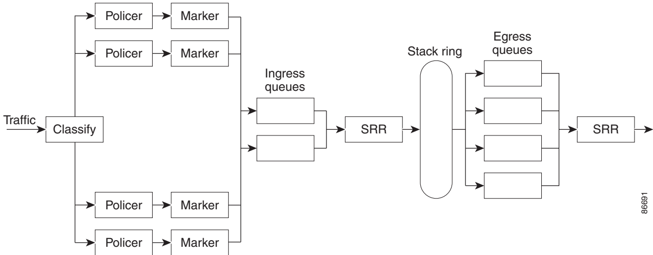
Figure 38-6 Ingress and Egress Queue Location on Catalyst 3750-E Switches
