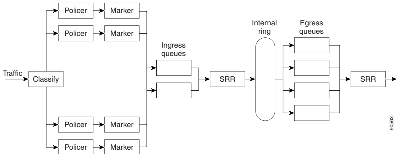
Figure 38-7 Ingress and Egress Queue Location on Catalyst 3560-E Switches
