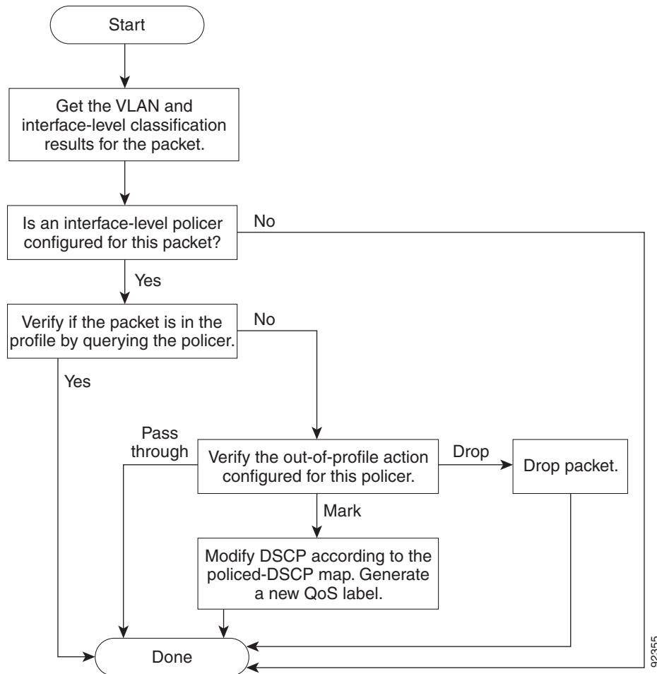
Figure 38-5 Policing and Marking Flowchart on SVIs
