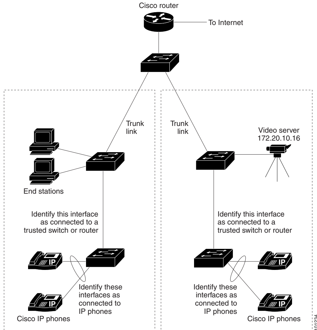
Figure 38-14 Auto-QoS Configuration Example Network
