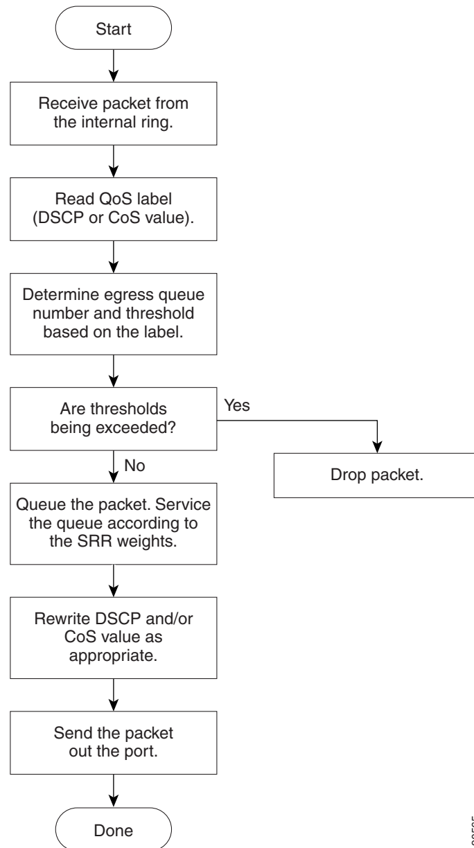
Figure 38-12 Queueing and Scheduling Flowchart for Egress Ports on Catalyst 3560-E Switches
