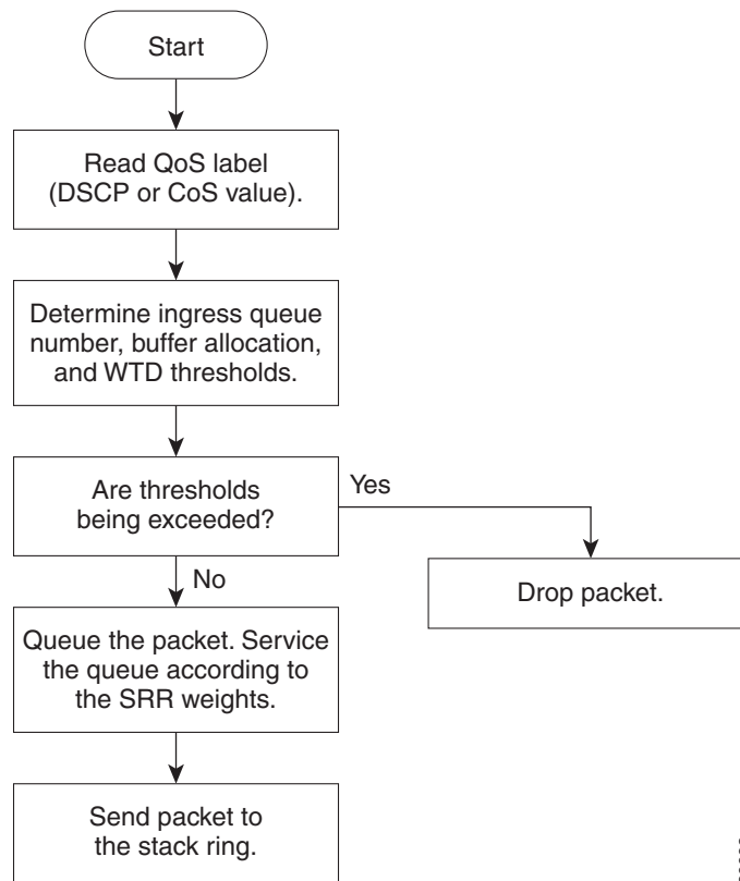
Figure 38-9 Queueing and Scheduling Flowchart for Ingress Ports on Catalyst 3750-E Switches
