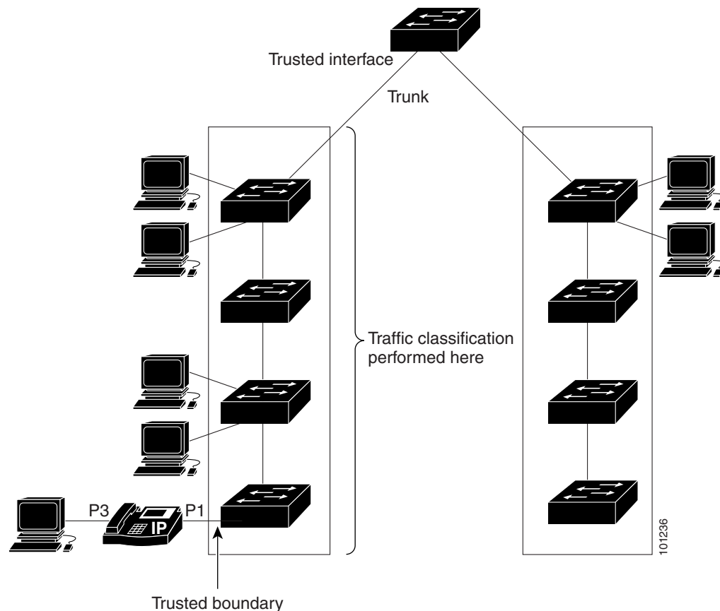
Figure 38-15 Port Trusted States within the QoS Domain
