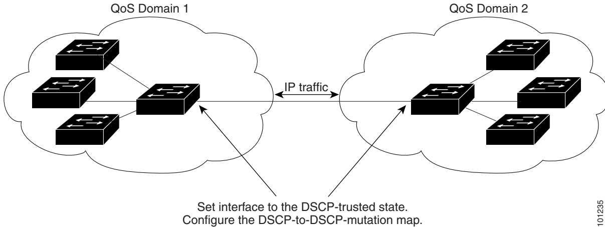
Figure 38-16 DSCP-Trusted State on a Port Bordering Another QoS Domain
