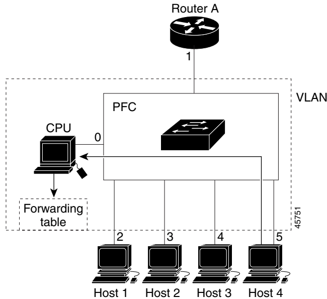
Figure 25-2 Second Host Joining a Multicast Group
