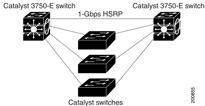
Figure 0-4 Redundant Gigabit Backbone
