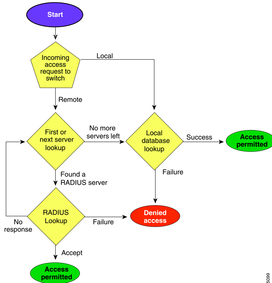
Figure 17-1 Authorization and Authentication Flow for User Login
