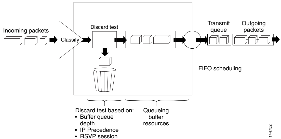
Figure 56-1 Weighted Random Early Detection
