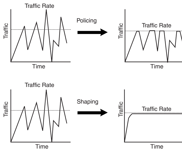
Figure 56-2 Traffic Policing vs. Traffic Shaping
