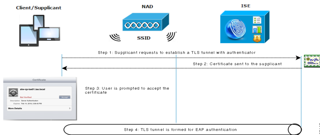
Figure E-2 EAP Communication
