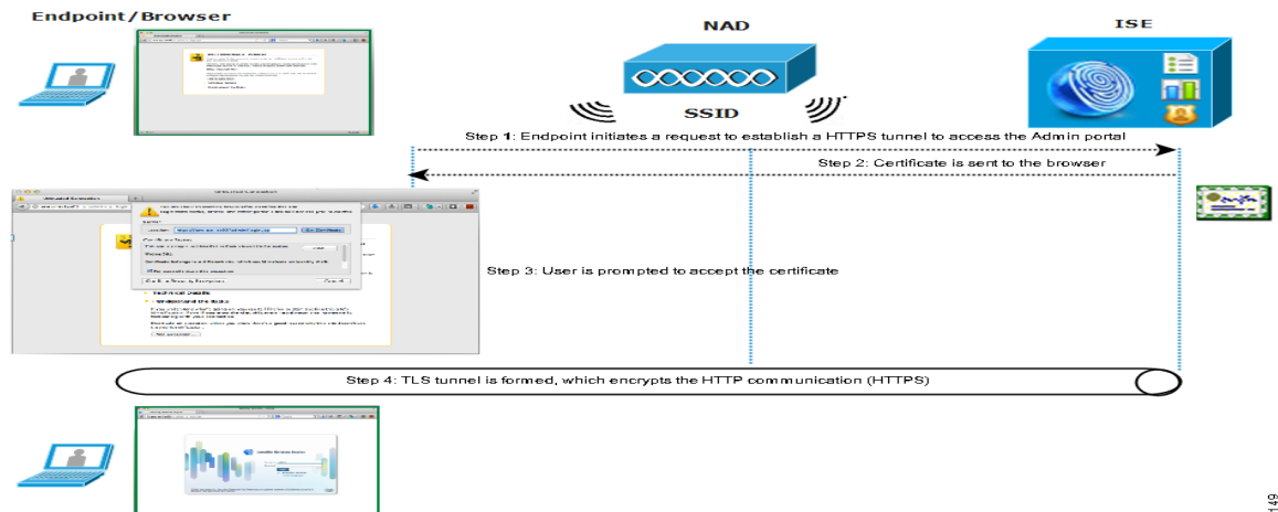
Figure E-1 HTTPS (TLS-Encrypted HTTP Communication)
