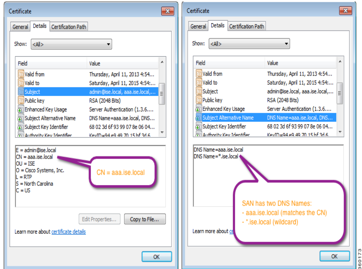
Figure E-3 Wildcard Certificate Example
