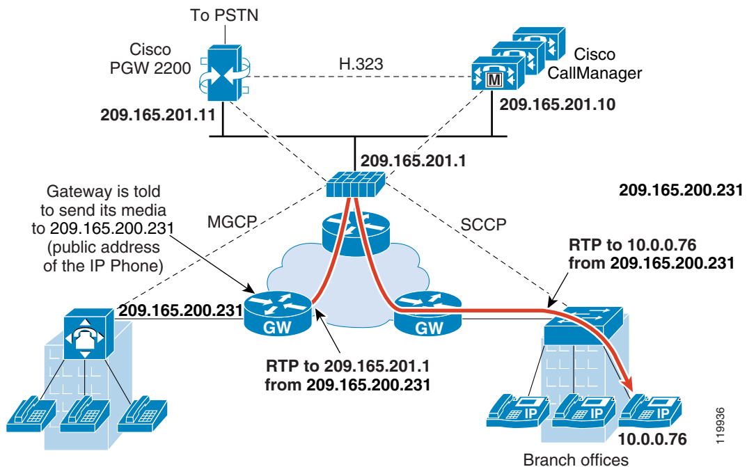
Figure 21-1 Using NAT with MGCP
