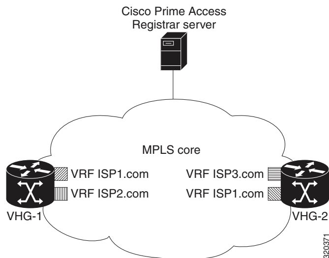
Figure 13-1 MPLS Core
