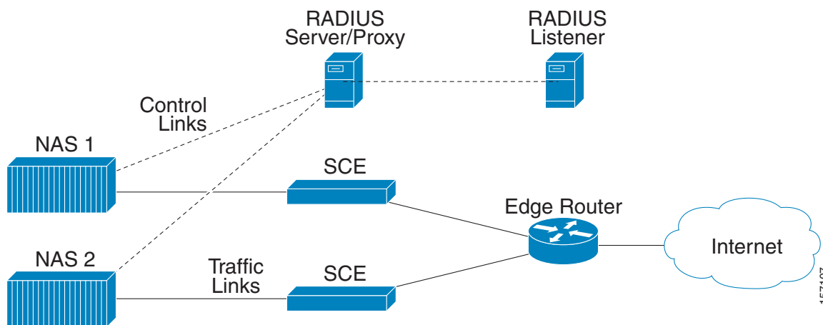
Figure 22-1 Example of when the only NAS that the RADIUS Listener is configured with is the Proxy Device
