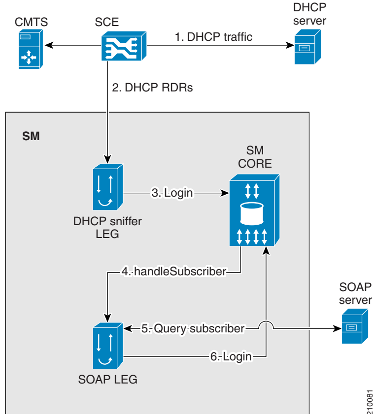
Figure 27-2 SOAP LEG Topology with DHCP Sniffer LEG
