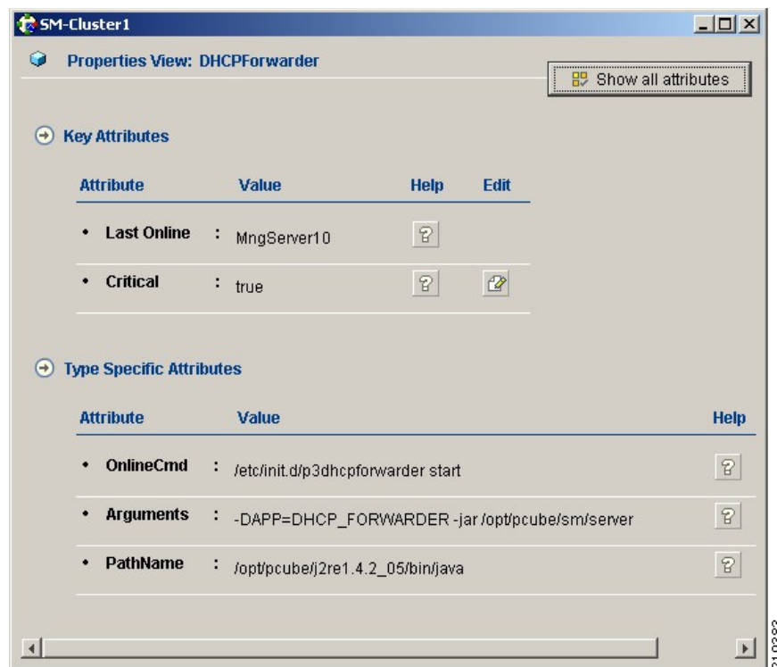
Figure 12-1 Adding a DHCP Forwarder Resource
