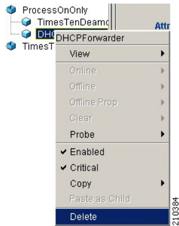
Figure 12-2 Removing a DHCP Forwarder Resource
