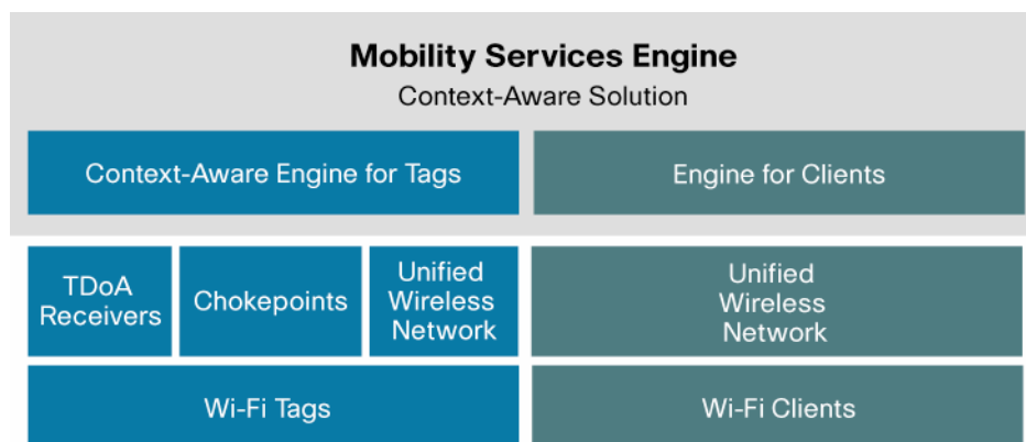
Figure 1. Context-Aware Software
