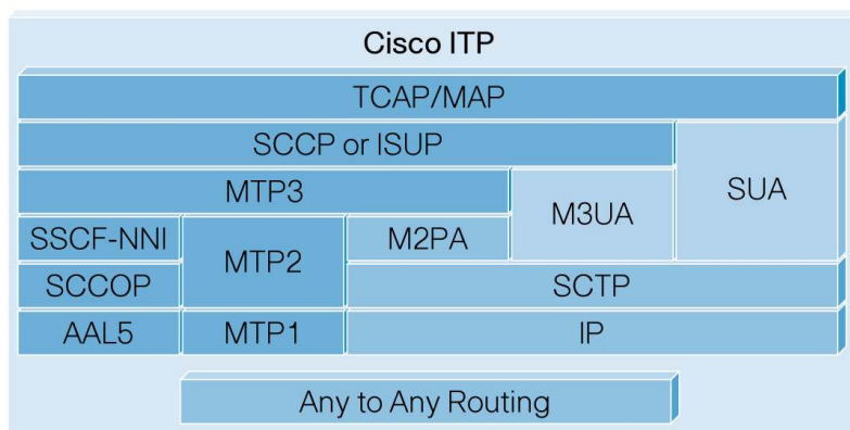
Figure 1. Cisco IP Transfer Point Protocol Architecture
