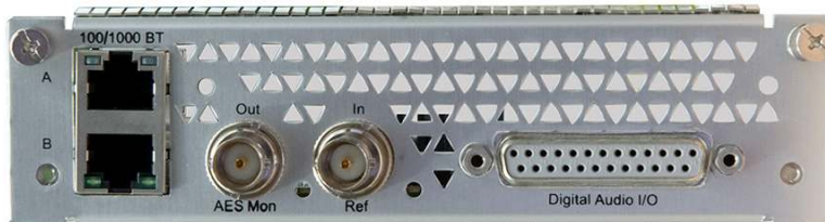
Figure 2. Cisco DCM Audio Gateway Rear Panel with the TASCAM SUB-D Interface
