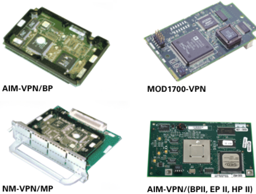
Figure 1 Cisco 1700, 2600, 3600 and 3700 Series VPN Modules
