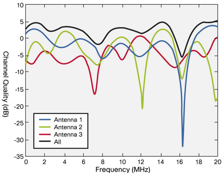
Figure 2. Variation of Signal Quality from Constructive and Destructive Interference across the Frequency Band of the Signal and across Antennas
