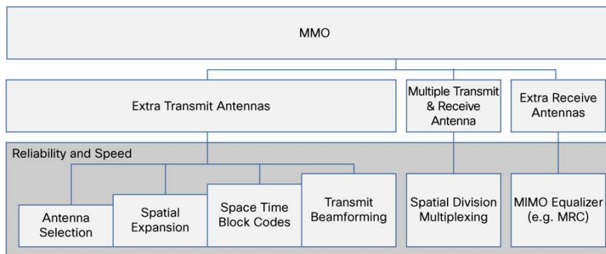
Figure 4. Reliability and Speed Improvements Enabled by MIMO
