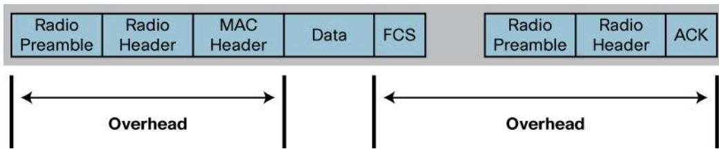
Figure 11. Overhead
