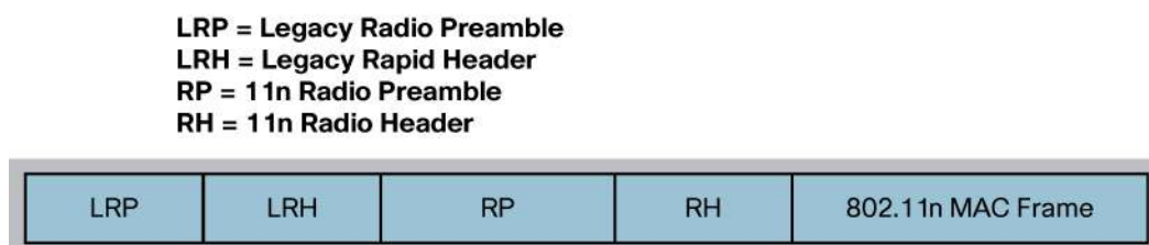
Figure 15. HT-Mixed Frame Format
