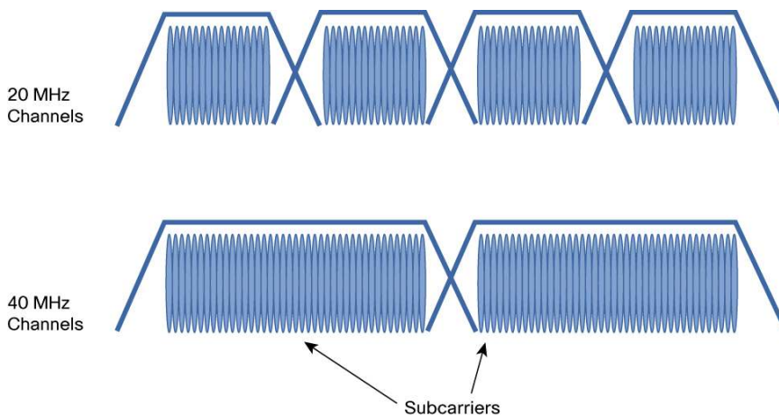
Figure 9. 20-MHz and 40-MHz Channels
