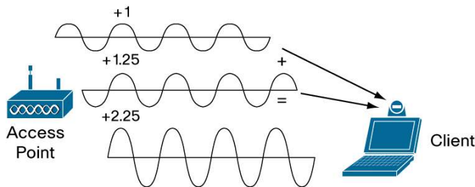
Figure 6. Transmit Beamforming (Synthesizing Constructive Interference)
