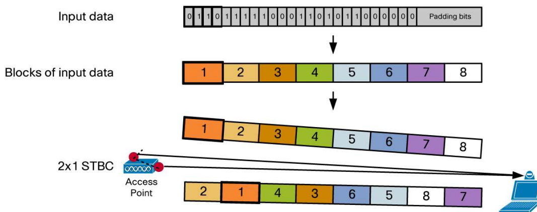
Figure 7. 2x1 STBC
